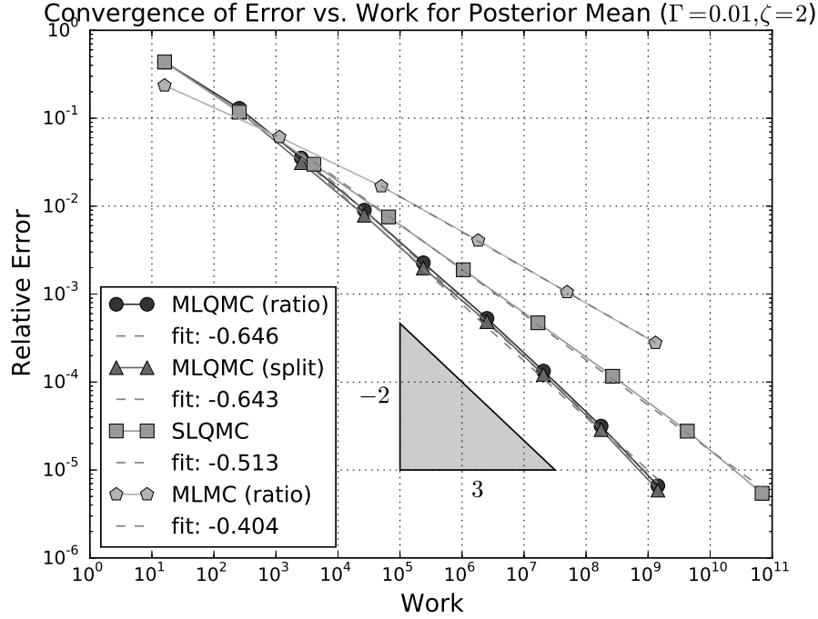
Figure 7: Convergence of estimates to the Bayesian inverse problem for the 2d diffusion equation model with coefficient (6.2), with \Gamma = 0.01 . The slope of the lines was estimated by a least-squares fit omitting the first three points.
