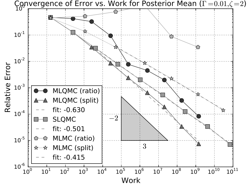
Figure 4: Convergence of estimates to the Bayesian inverse problem for the affine-parametric 2d diffusion equation model, with covariance \Gamma = 0.01 . The slope of the lines was estimated by a least-squares fit omitting the first three points. In this case, the MLQMC splitting estimator was used as a reference. In the small noise case, the convergence of the ratio estimator is negatively impacted, both for MLMC and for MLQMC. The splitting estimator seems to be more resilient for small \Gamma , as indicated in Remark 4.1.
