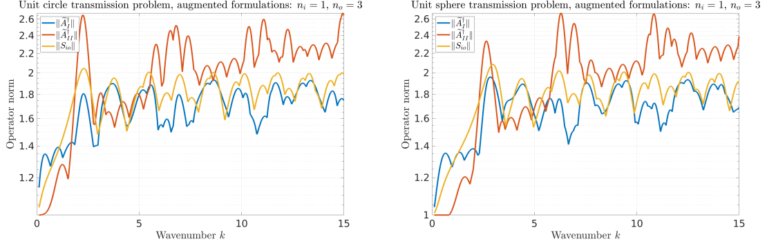
Figure 3: Plots of the operator norms of the pseudo-inverses \tilde{A}_I^\dagger , \tilde{A}_{II}^\dagger of the augmented BIOs
