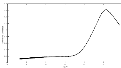
(D) Symmetric differences as a function of \log(J) .
