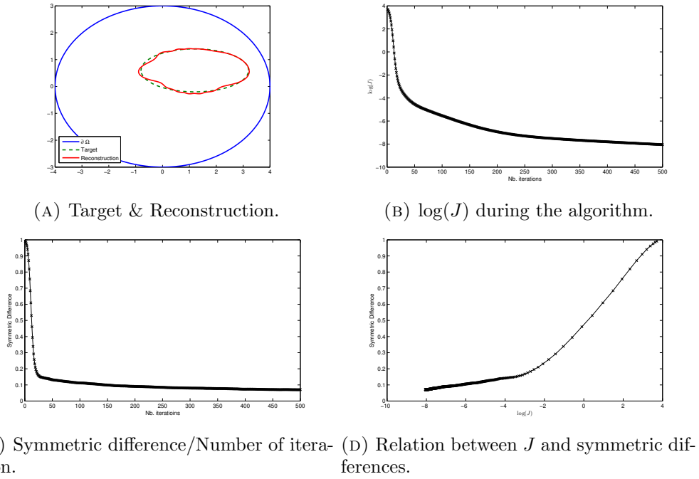
FIGURE 1. Exemple 1: ellipse
