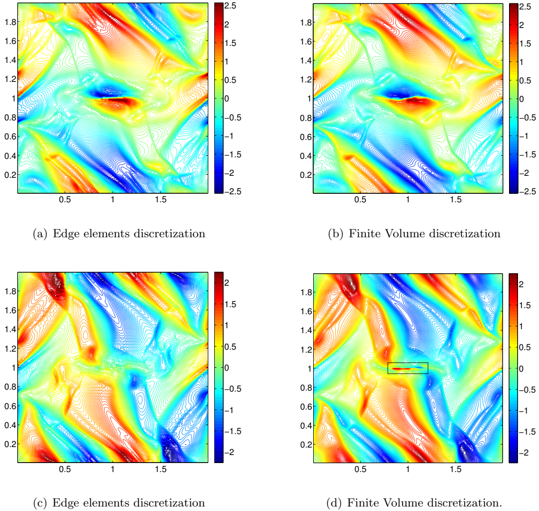
Figure 6.10: Orszag-Tang benchmark: Comparison at time T = 1 between the magnetic potential obtained with the stabilized scheme (2.7)-(2.8), lowest order edge elements and second order Heun time-stepping (first column (a)-(c)) and the corresponding components of the magnetic field obtained from the MHD simulation with a finite volume scheme in [21] (second column (b)-(d)). The current sheet in Figure (d) is framed in the black box.
