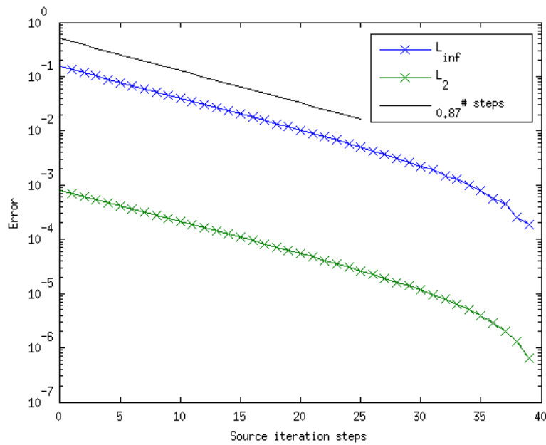
(b) Convergence for \sigma = 0.5
