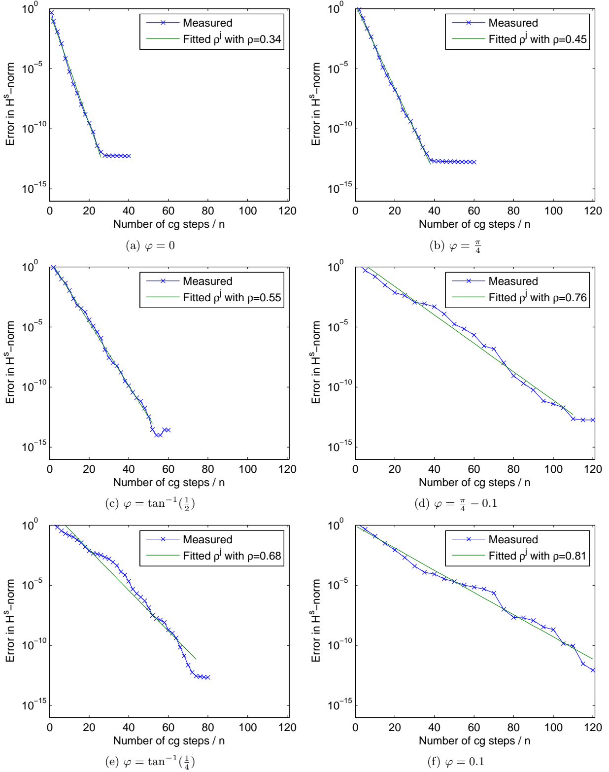
Figure 5.1: Convergence of CG applied to the ridgelet space RTE (4.6) using J = 4 , \vec{s} = (\cos(\varphi), \sin(\varphi))^\top , \kappa = 1 and f(x, y) = e^{-100((x-0.5)^2 + (y-0.5)^2)} . The error was measured in the H^{\vec{s}} -norm, compare Definition 4.2.1.
