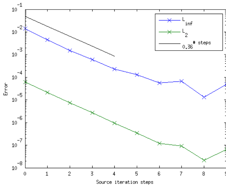
(a) Convergence for \sigma = 0.2
