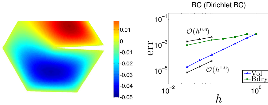
Fig. 4.3 Plot of the solution u of the state problem in the computational domain \Omega (left) for the third numerical experiment , and corresponding convergence study (right). Due to the poor regularity of the functions u and p , the convergence rate of d\mathcal{J}(\Omega, u_h, p_h; \mathcal{V})^{\text{Vol}} and d\mathcal{J}(\Omega, u_h, p_h; \mathcal{V})^{\text{Bdry}} deteriorate.
