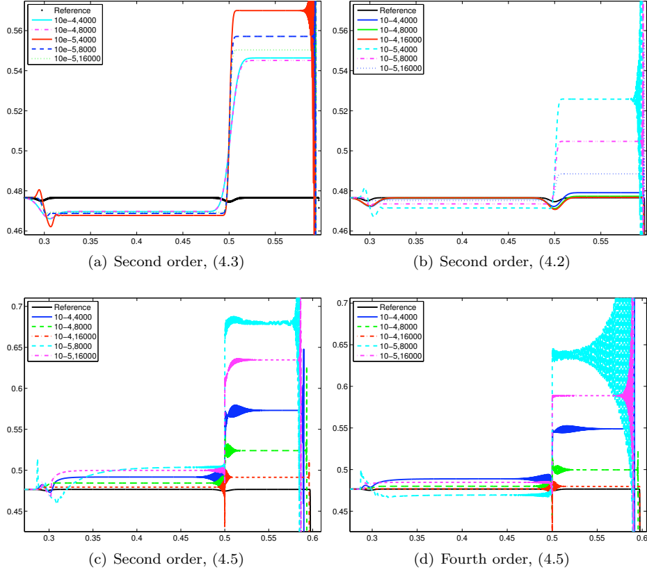
FIGURE 3. Computed density for (3.12) with different regularizations of the non-conservative system (2.5). In each plot, the value of the viscosity coefficient and the number of mesh points are indicated.
