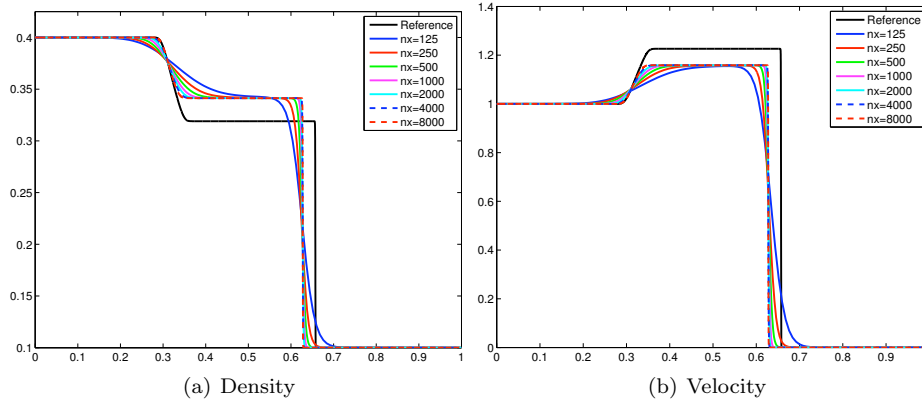
FIGURE 8. Solution computed with the ELF scheme.
