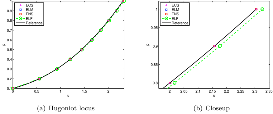
FIGURE 6. The numerical Hugoniot locus in the u - p plane computed with the ECS, ELF, ELM and ENS schemes.
