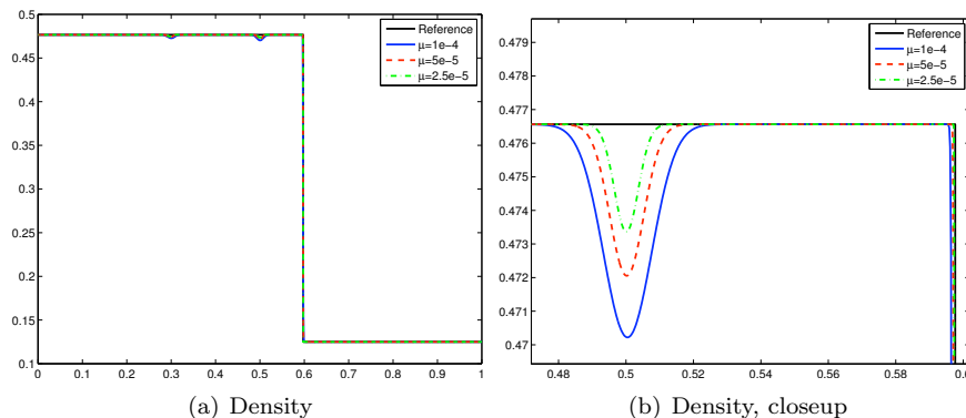
FIGURE 2. Computed solution for the Riemann problem (3.12) for the viscous equation (4.1) with a second-order scheme.
