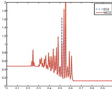
FIGURE 1. Computed density for the Riemann problem (3.12) with the EC2 and NEC2 schemes at time t = 0.25 on a mesh with 200 points.
