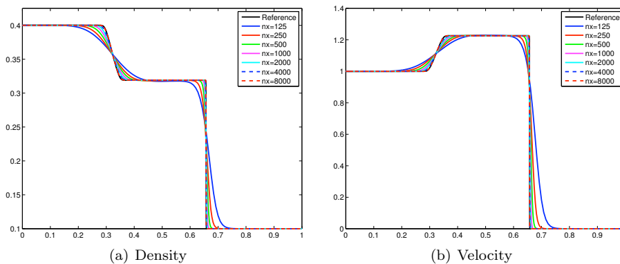
FIGURE 9. Solution computed with the ELM scheme.
