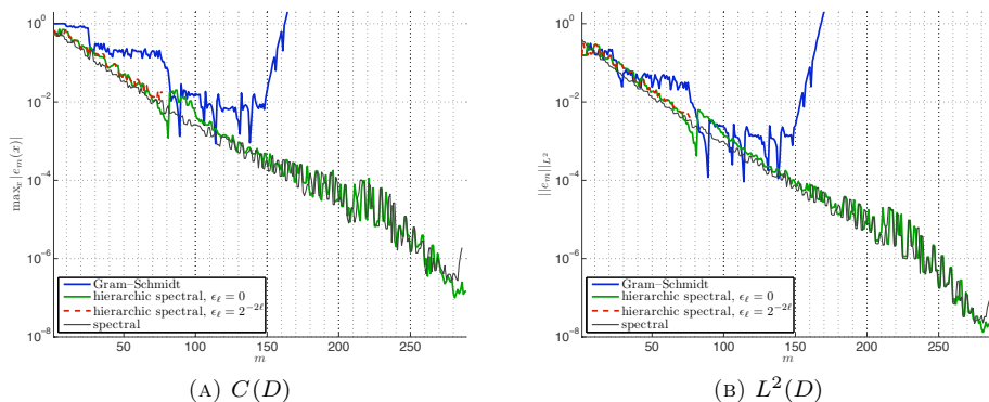
FIGURE 4.10. decay of the basis functions for d = 2
