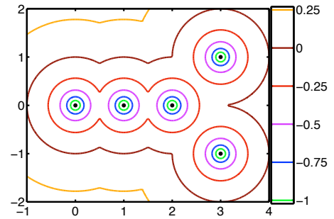
(a) Unstructured pseudospectrum
