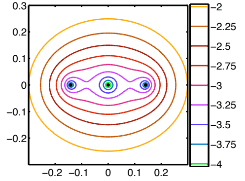
(a) Unstructured pseudospectrum
