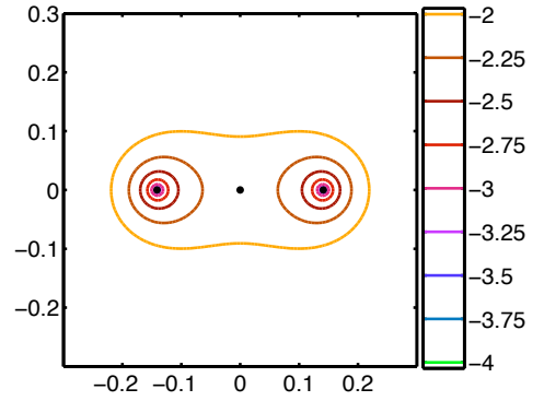
(b) Skew-symmetric pseudospectrum
