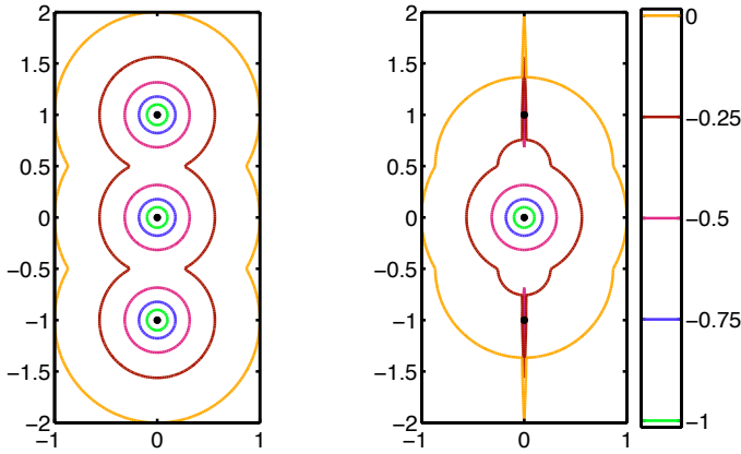
(a) Unstructured pseudospectrum (b) Hamiltonian pseudospectrum
