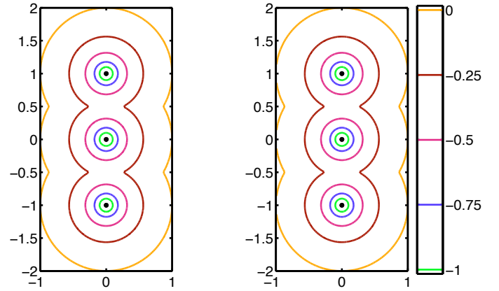
(a) Unstructured pseudospectrum (b) Hamiltonian pseudospectrum
