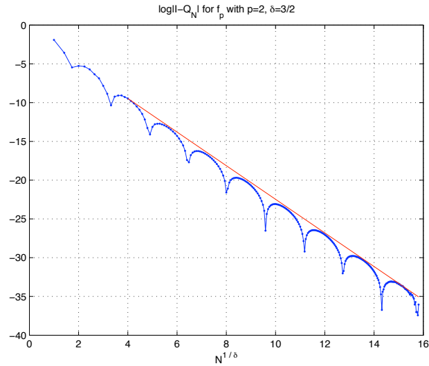
FIGURE 6.1. \log |\mathcal{I}f_p - Q_N f_p| for function f_p in (6.1) with p = 2 , \delta = \frac{3}{2} and N = 1, \dots, 250 . The horizontal axis is N^{1/\delta} , the line corresponds to |\mathcal{I}f_p - Q_N f_p| = C \exp(-rN^{1/\delta}) .
