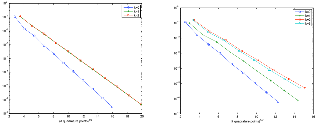
FIGURE 6.2. Relative errors |Q_N - I|/I for d = 2 (left) and d = 3 (right), with k = 0, \dots, d
