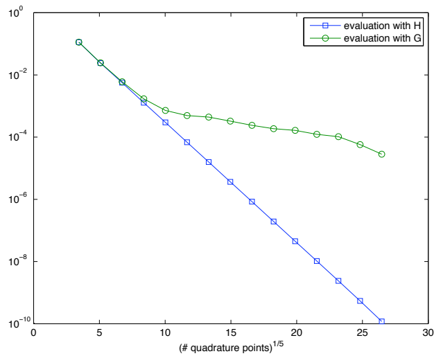
FIGURE 6.3. Relative error |\mathcal{Q}_N - I|/I for naive evaluation of integrand G and improved algorithm evaluating H
