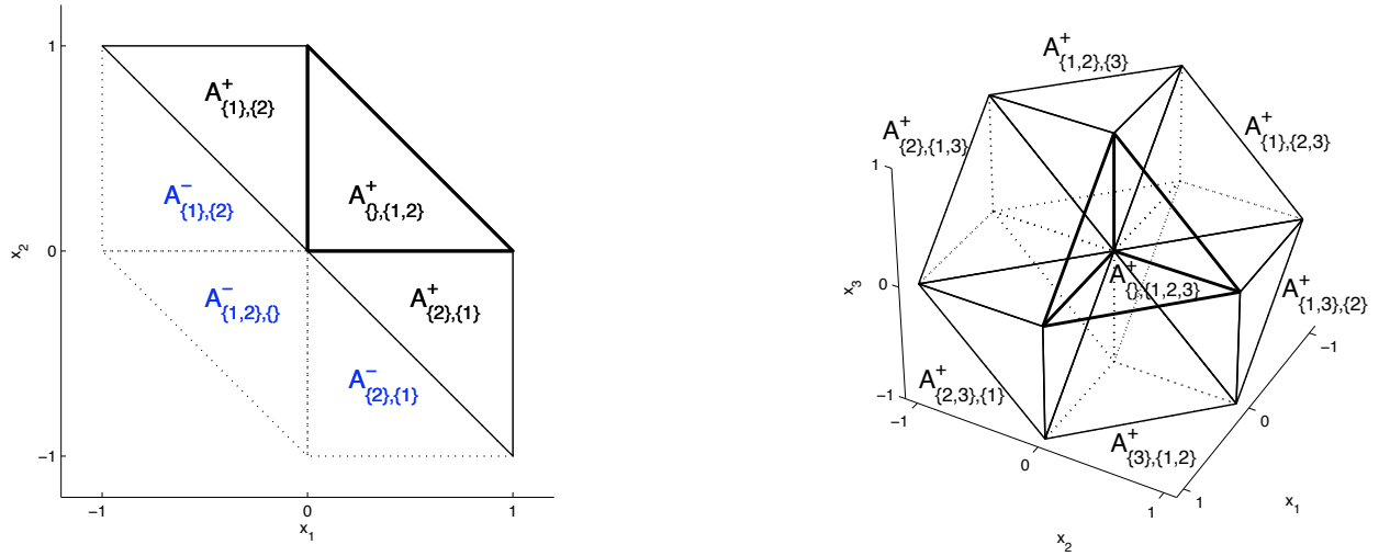
FIGURE 3.1. The domain A_d = \bigcup_{N \subset M} \bigcup_{\sigma \in \{+, -\}} A_{N, M \setminus N}^\sigma for d = 2 (left) and d = 3 (right, only labeled for \sigma = + )
