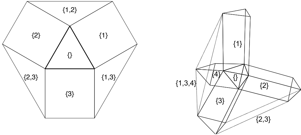
FIGURE 3.2. The bases B_{N,M\setminus N}^+ flattened into \mathbb{R}^{d-1} for d = 3 (left) and d = 4 (right) and labeled with N . For d = 4 only 1 of 6 bases with \#N = 2 and 1 of 4 bases with \#N = 3 are shown with dotted lines.
