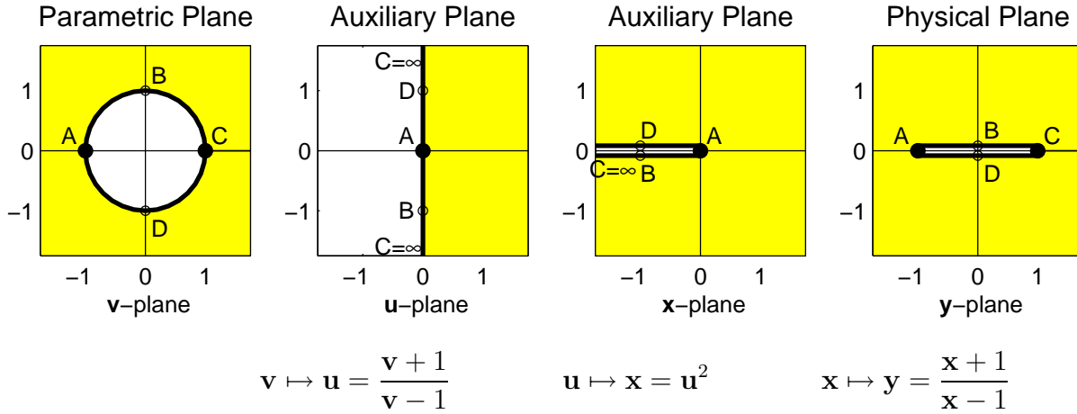
Figure 2: The sequence of conformal mappings generating the planar Birkhoff transformation
