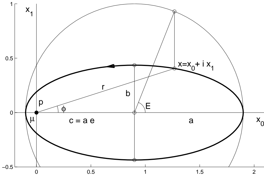
Figure 1: The planar elliptic Kepler motion with eccentricity e = 0.9 . a, b semi-axes, c focal distance, p semi-latus rectum, E eccentric anomaly, \mu gravitational parameter, r distance, \phi polar angle
