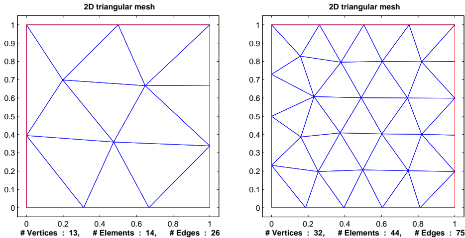
FIG. 7.1. The third and fifth coarsest meshes on the unit square.
