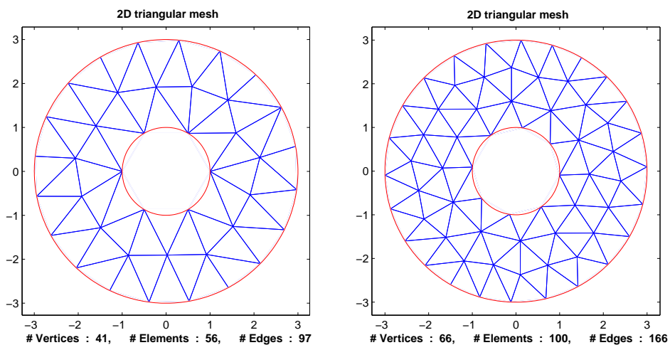
FIG. 7.7. Experiment 2: the two coarsest meshes on the annulus.
