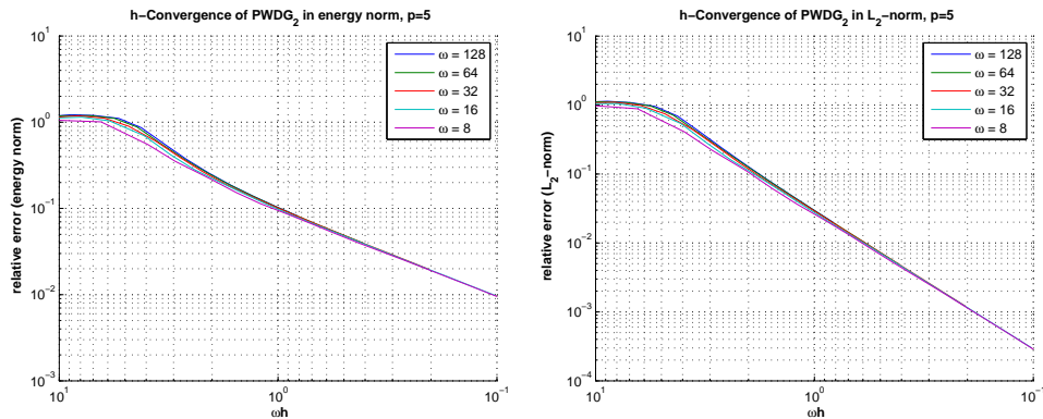
FIG. 7.14. Experiment 3: h -convergence of PWDG2 for various values of \omega . The relative errors in the energy norm (7.2) and the L^2 -norm are plotted against \omega h .
