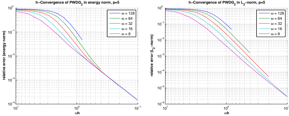
FIG. 7.5. Experiment 1: h-convergence of PWDG2 for various values of \omega . The relative errors in the energy norm (7.2) and the L^2 -norm are plotted against \omega h .
