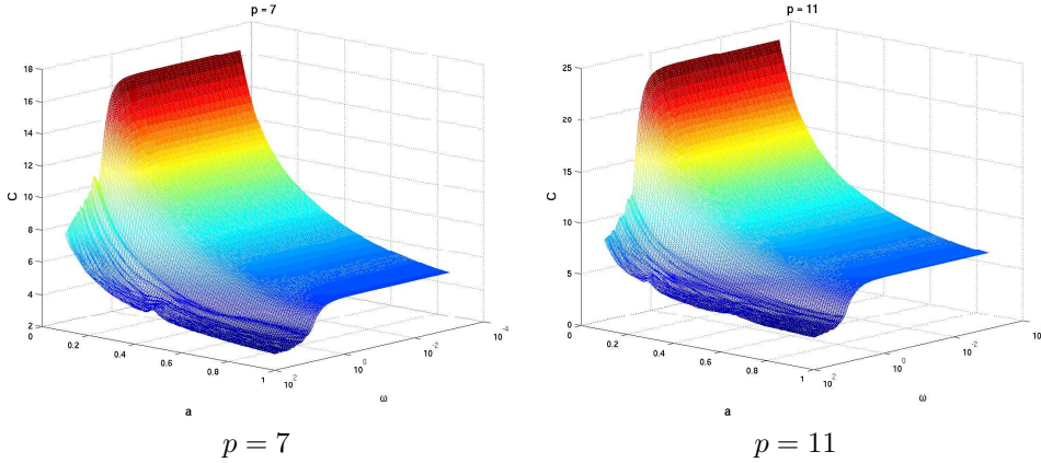
FIG. 4.4. Constants in the inverse trace norm inequality for triangle with vertices (0, 0), (1, 0), (0, a) , a > 0 .
