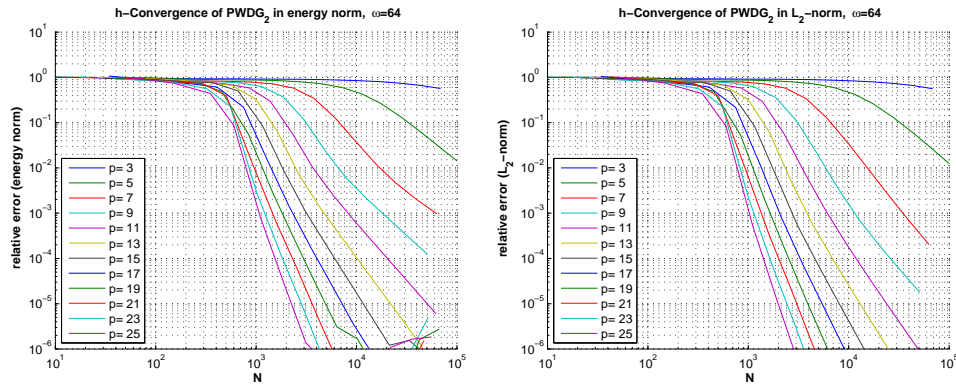
FIG. 7.4. Experiment 1: h -convergence of PWDG2 for various values of p . The relative errors in the energy norm (7.2) and the L^2 -norm are plotted against the number N of degrees of freedom.
