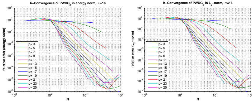
FIG. 7.10. Experiment 2: h -convergence of PWDG2 for various values of p . The relative errors in the energy norm (7.2) and the L^2 -norm are plotted against the number N of degrees of freedom.
