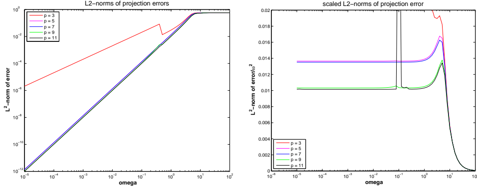
FIG. 4.7. L^2 projection error onto plane wave space for linear function x . The wiggles at \omega = \frac{1}{2} reflect the truncation error for the stable basis.
