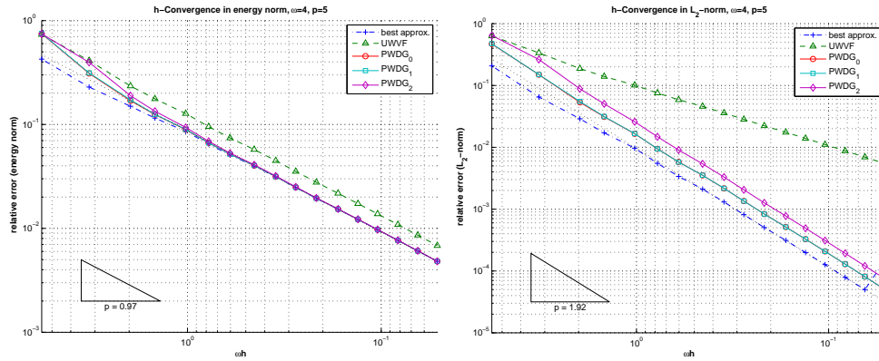
FIG. 7.11. Experiment 3: h -convergence of PWDG methods for \omega = 4 . The relative errors in the energy norm (7.2) and the L^2 -norm are plotted against \omega h .
