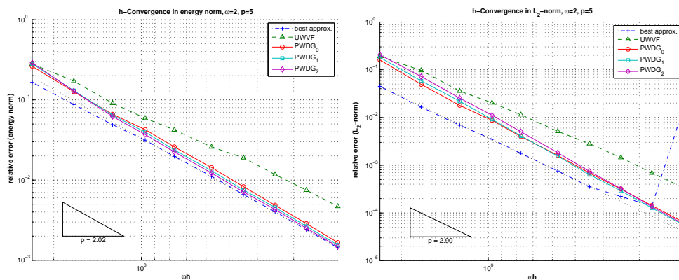
FIG. 7.8. Experiment 2: h -convergence of PWDG methods for \omega = 2 . The relative errors in the energy norm (7.2) and the L^2 -norm are plotted against \omega h .
