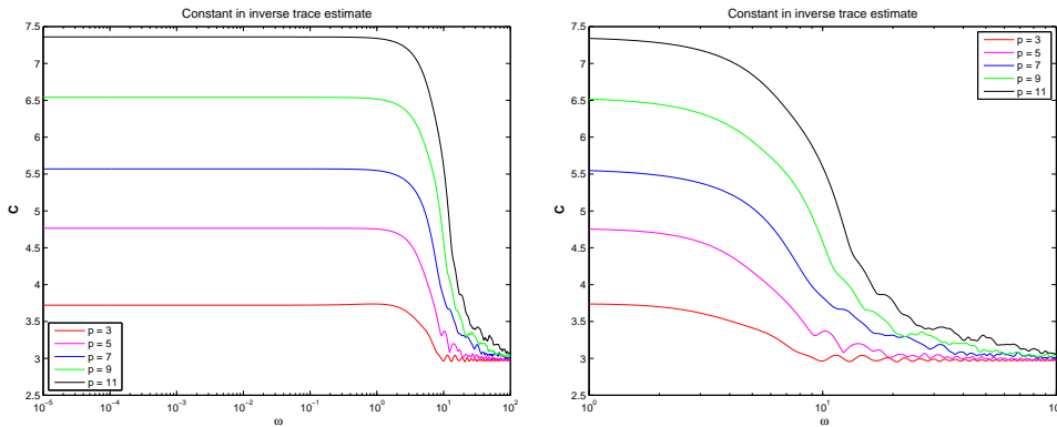
FIG. 4.3. Constants in the inverse trace norm inequality of Theorem 4.7 for the unit triangle
