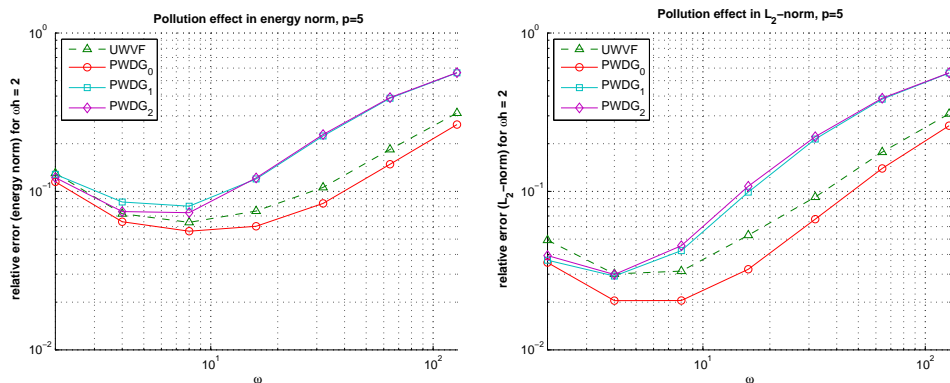
FIG. 7.6. Experiment 1: errors of PWDG methods for fixed \omega h = 2 and variable \omega . Values were computed by linear interpolation (w.r.t. h ) of data points in bilogarithmic scale.
