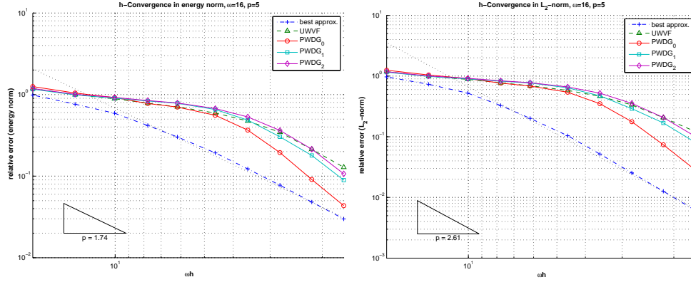
FIG. 7.9. Experiment 2: h -convergence of PWDG2 for \omega = 16 . The relative errors in the energy norm (7.2) and the L^2 -norm are plotted against \omega h .
