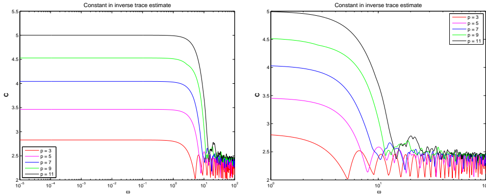
FIG. 4.2. Constants in the inverse trace norm inequality of Theorem 4.7 for K = ]0, 1[^2
