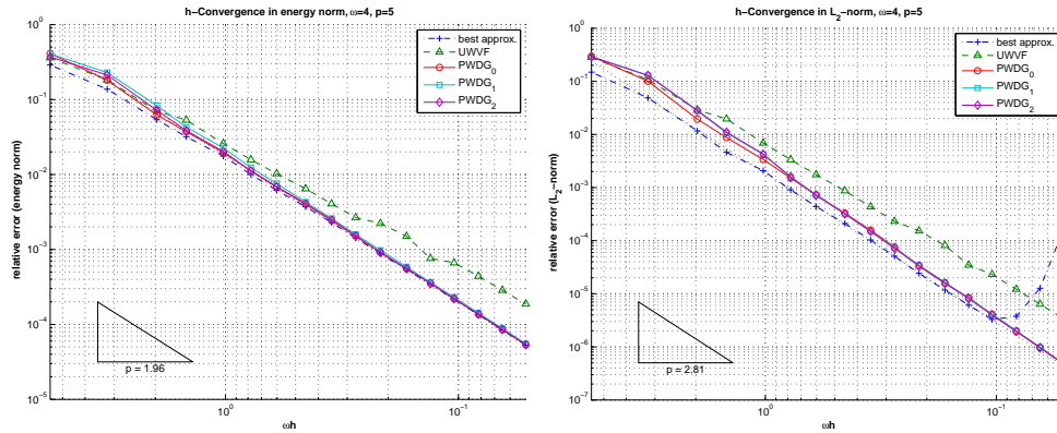
FIG. 7.2. Experiment 1: h -convergence of PWDG methods for \omega = 4 . The relative errors in the energy norm (7.2) and the L^2 -norm are plotted against wh . The divergence of the best approximation in the L^2 -norm is due to numerical instability in the computation of the L^2 -projection.
