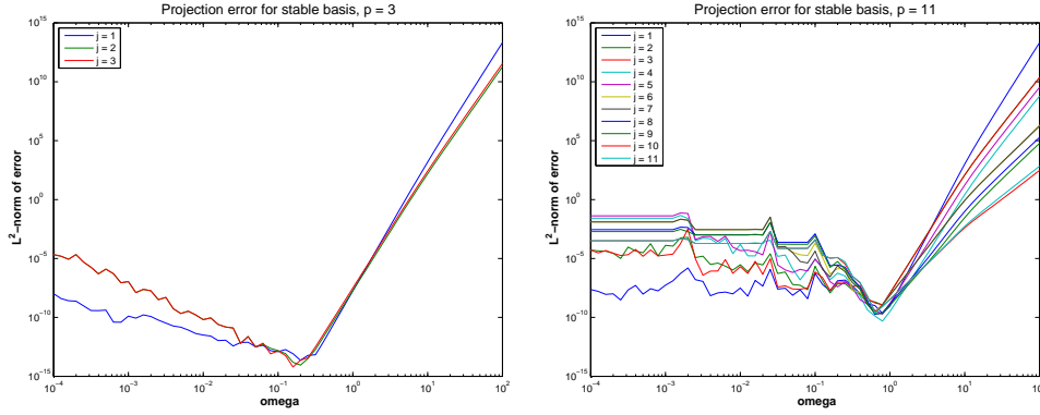
FIG. 4.1. Residual norm for L^2 projection of truncated basis functions b_j onto plane wave space. Truncation after 13 terms in the expansion w.r.t. \omega .
