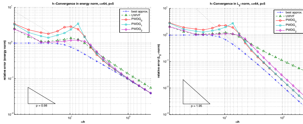
FIG. 7.12. Experiment 3: h -convergence of PWDG methods for \omega = 64 . The relative errors in the energy norm (7.2) and the L^2 -norm are plotted against \omega h .
