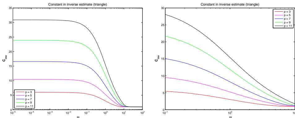
FIG. 4.6. Constant in inverse inequality of Thm. 4.8 for the unit triangle
