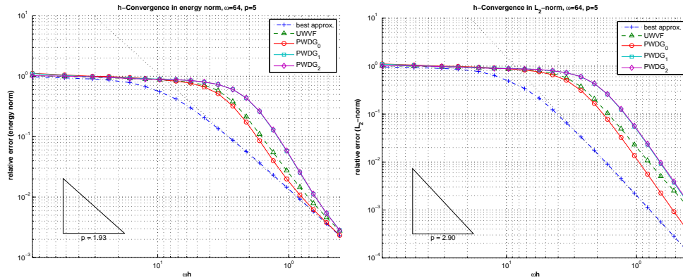
FIG. 7.3. Experiment 1: h -convergence of PWDG methods for \omega = 64 . The relative errors in the energy norm (7.2) and the L^2 -norm are plotted against wh .
