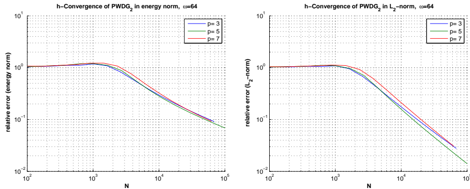
FIG. 7.13. Experiment 3: h -convergence of PWDG2 for various values of p . The relative errors in the energy norm (7.2) and the L^2 -norm are plotted against the number N of degrees of freedom.
