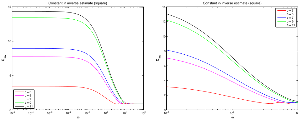
FIG. 4.5. Constant in inverse inequality of Thm. 4.8 for K = ]0, 1]^2
