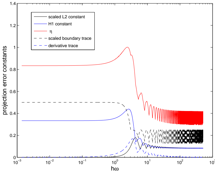
FIG. 6.1. Function \eta from (6.17)
