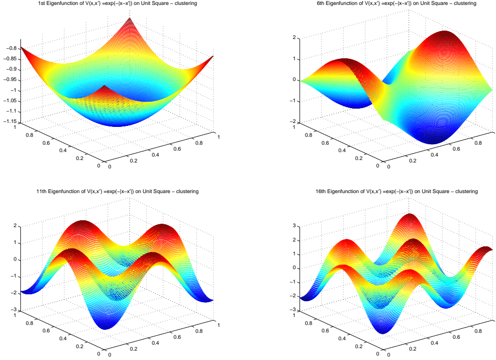
Figure 4.2: Eigenfunctions No. 1,6,11,16 of exponential covariance kernel ((4.20) with \delta = 1, C = 1 ) on unit square D = ]0, 1[^2 for correlation length 1, computed using clustering on a regular triangulation of D with 32768 triangular elements. PC w. 1GB RAM, generalized FMM and [9] was used.
