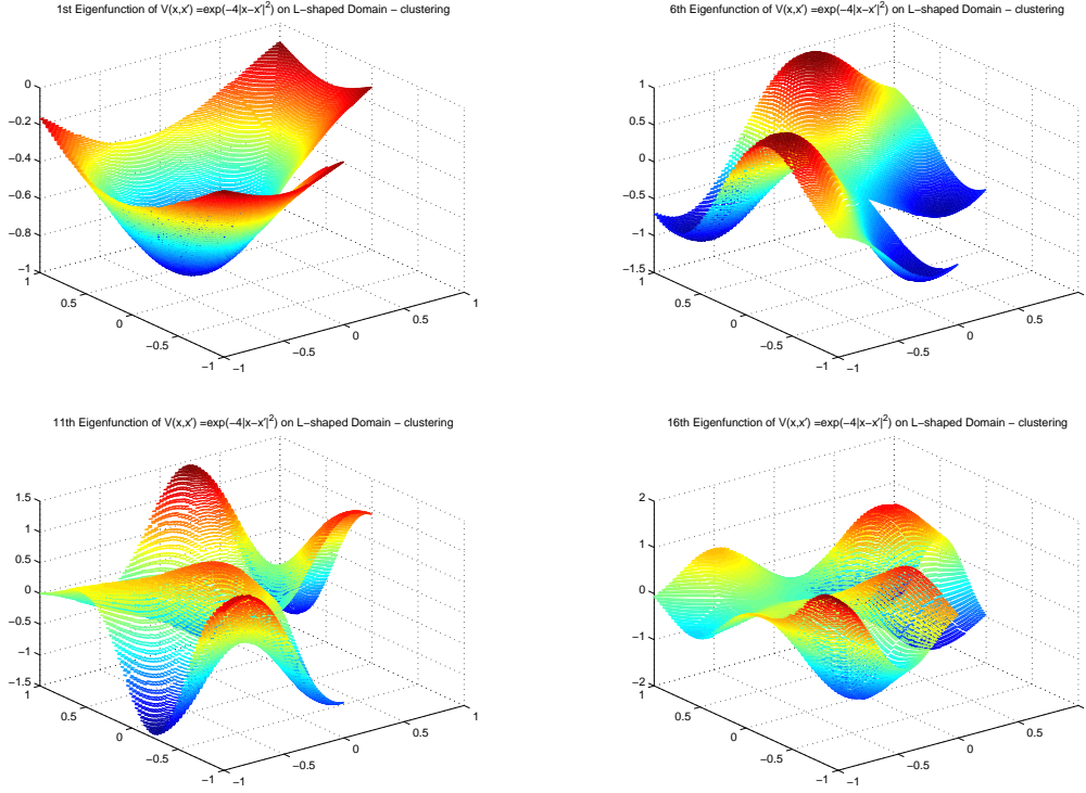
Figure 4.1: Eigenfunctions No. 1,6,11,16 of Gaussian covariance kernel ((4.20) with \delta = 2, C = 1 ) on L-shaped domain D = ]-1, 1[^2 \setminus ([0, 1] \times [-1, 0]) for correlation length 0.5, computed using clustering on a regular triangulation of D with 16384 triangular elements. PC w. 1GB RAM, generalized FMM and [9] was used.
