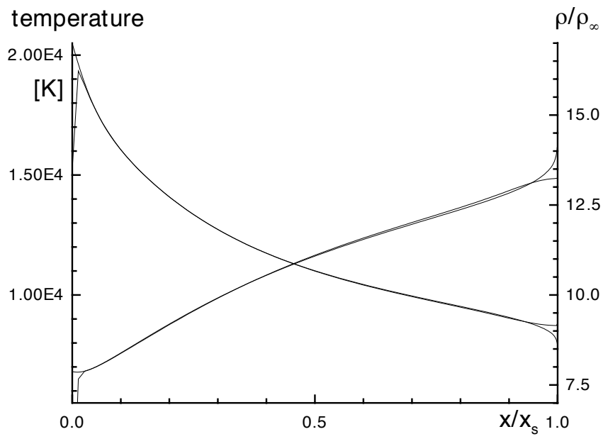
Figure 11: Comparison of solutions of BVP and 2D calculation with standard van Leer scheme
