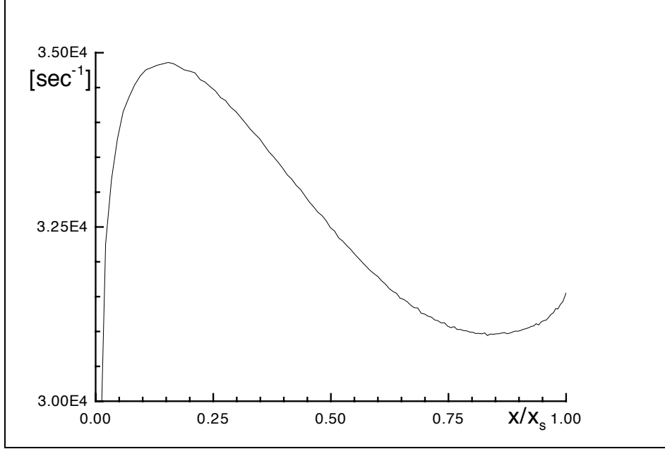
Figure 2: v_y along the stagnation streamline
