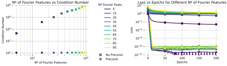
Figure 7.1. Poisson equation with Fourier features. Left : Optimal condition number vs. Number of Fourier features. Right : Training for the unpreconditioned and preconditioned Fourier features. Figure from De Ryck et al. (2023a).
