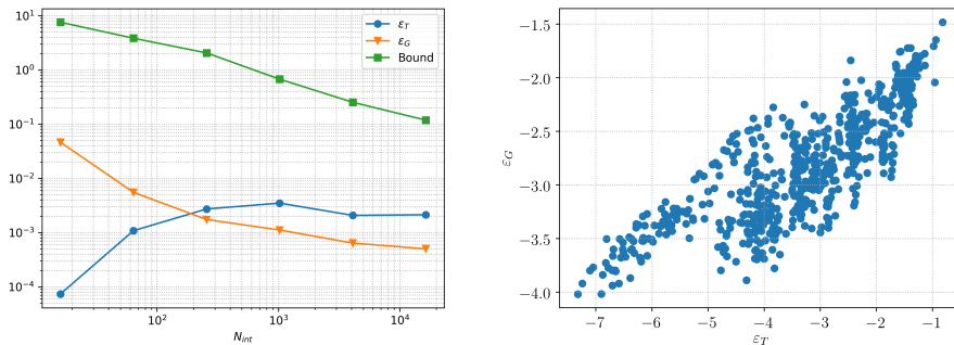
Figure 6.2. Experimental results for the heat equation. The generalization error \mathcal{E}_G and the training error \mathcal{E}_T are shown in terms of the number of residual points N_{\text{int}} ( left ; and compared with the bound from Theorem 6.7) and also in terms of each other ( right ). Figure from Molinaro (2023).
