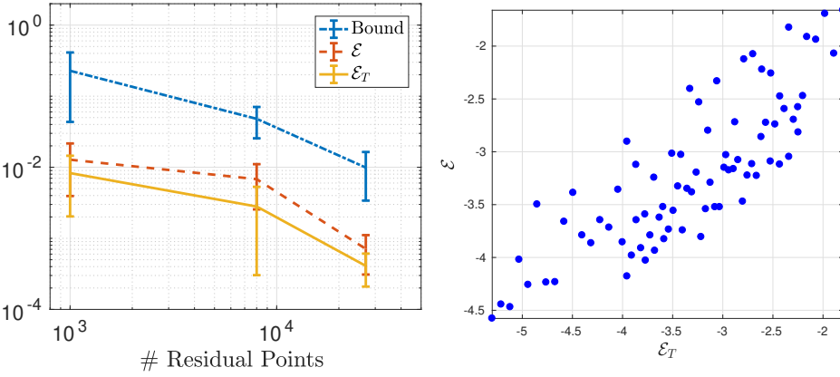
Figure 6.1. Experimental results for the Navier-Stokes equation with \nu = 0.01 . The total error \mathcal{E} and the training error \mathcal{E}_T are shown in terms of the number of residual points N_{\text{int}} (left; and compared with the bound from Theorem 6.5) and also in terms of each other (right). Figure from De Ryck et al. (2023b).
