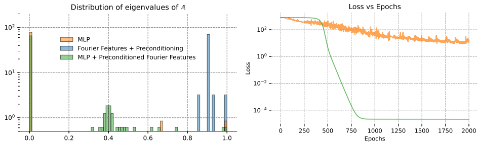
Figure 7.3. Poisson equation with MLPs. Left : Histogram of normalized spectrum (eigenvalues multiplied with learning rate). Right : Loss vs. number of epochs. Figure from De Ryck et al. (2023a).
