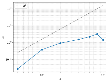
Figure 6.3. Relative generalization error \mathcal{E}_G (in percent) in terms of the parameter dimension d for the heat equation with a parametrized initial condition. Figure from Molinaro (2023).
