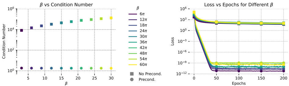
Figure 7.2. Linear advection equation with Fourier features. Left : Optimal condition number vs. \beta . Right : Training for the unpreconditioned and preconditioned Fourier features. Figure from De Ryck et al. (2023a).
