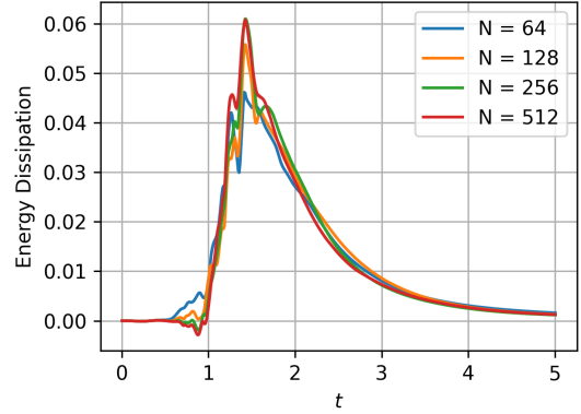
Figure 6: Evolution of energy dissipation -\frac{dE}{dt} in the Taylor-Green vortex experiment. Visually, there seems to be a good agreement with energy dissipation rates commonly found in literature [7].
