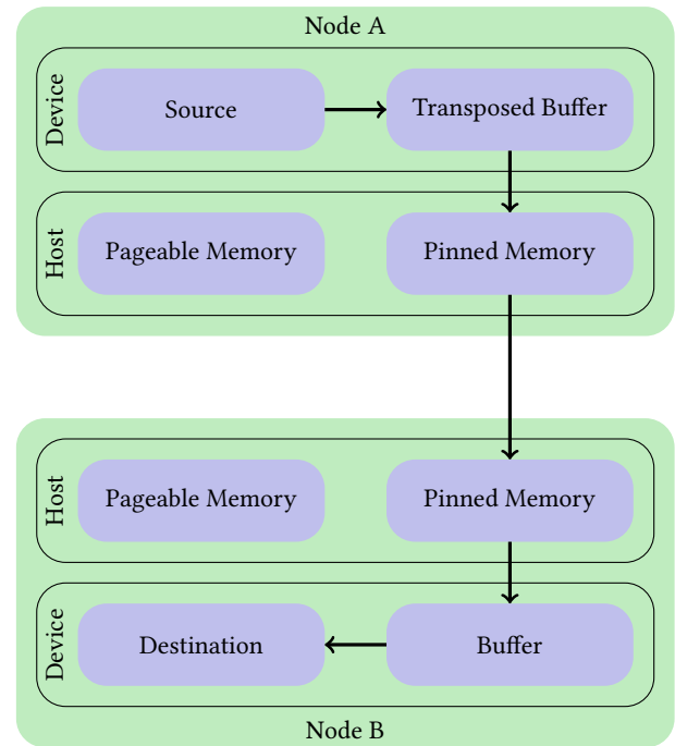
Figure 2: Unidirectional datapath between two nodes for the distributed transpose operation on GPUs. We first preprocess the data by transposing it locally on the GPU. This data is then copied down into pinned memory on the host bypassing pageable memory doubling the bandwidth for device to host transfers. This is followed by sending the data asynchronously over MPI to the receiving node. There, the data is received directly into another pinned memory block and consequently copied onto the GPU. Finally, the data is then distributed into the destination array containing the transposed data.
