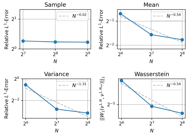
Figure 7: Convergence rates under mesh refinement of a single sample (top left), the mean (top right), the variance (bottom left), and the 1-point Wasserstein distance (bottom right) for the Taylor-Green Vortex. As expected, no sample wise convergence can be observed which can be explained by the ever smaller vortices being resolved and influencing the larger scales of the flow. Nevertheless, the pointwise mean and variance both seem to converge with a reasonable rate. This is confirmed by the convergence in the Wasserstein distance of the one-point correlation marginals of the statistical solution.
