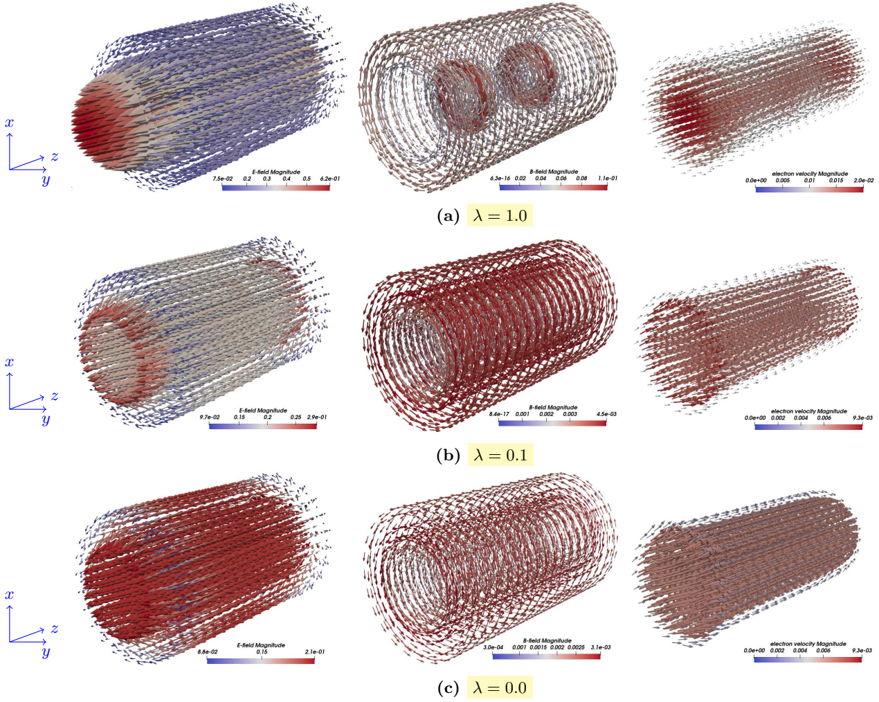
Fig. 9. Case II: Snapshots of the \mathbf{E} -field, \mathbf{B} -field, and \mathbf{u}_e for different \lambda at t = 10 based on a primal mesh with 1920 cells (16 cells along z -axis).
