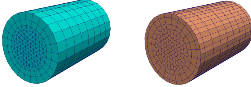
Fig. 5. Primal mesh (left) and dual mesh (right).
