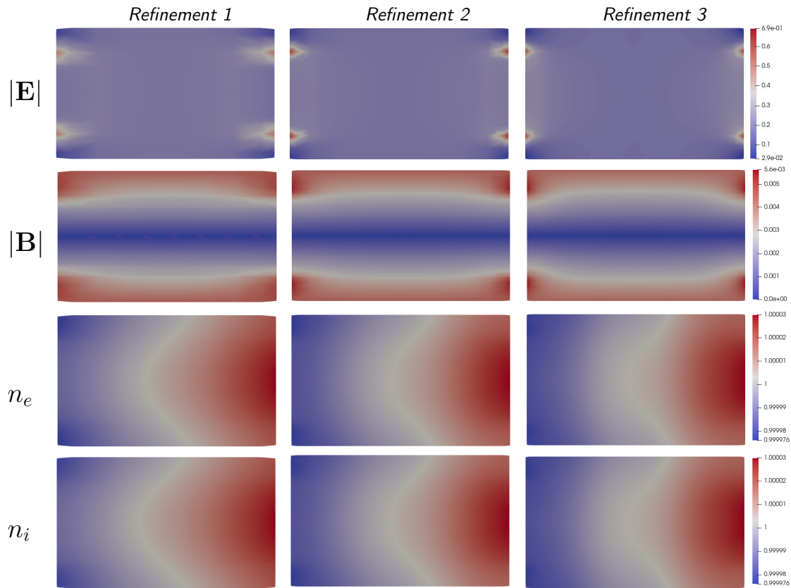
Fig. 11. Case II: Computed quantities at a cross-section on meshes on different refinement levels. Refinement 1: 1920 primal cells; Refinement 2: 14592 primal cells; Refinement 3: 30720 primal cells. The snapshots are computed for \lambda = 0 at t = 1 .
