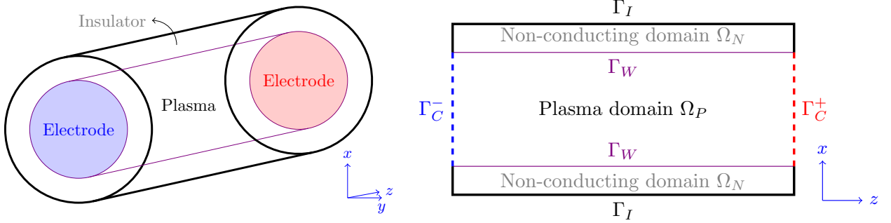
Fig. 2. The right figure shows the cross section in the x - z plane and the different parts of the boundary and interfaces.
