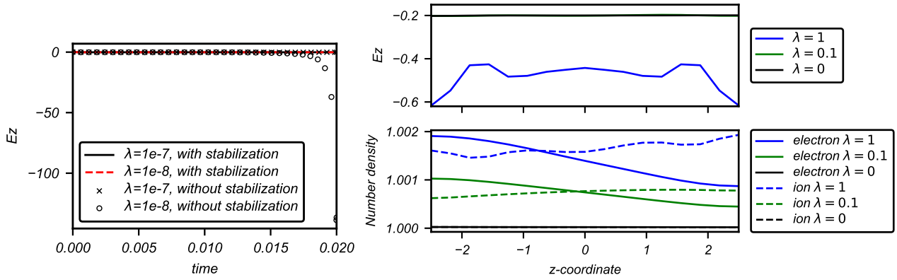
(a) time-dependent z -component of the \mathbf{E} -field in a boundary cell on \Omega_N (b) Quantities along z -axis for different \lambda ; the results are computed at t = 10 on a mesh with 1920 primal cells and 8 layers along z -axis.
