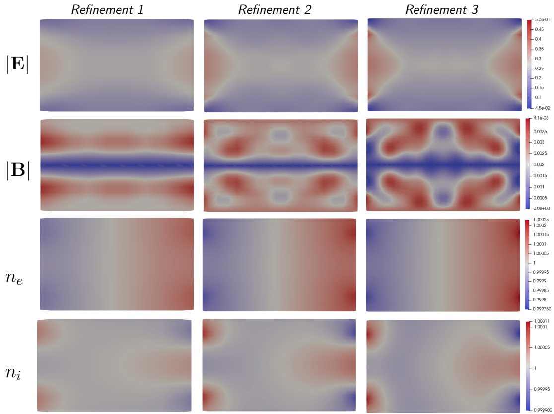
Fig. 10. Case II: Computed quantities at a cross-section on meshes with different refinement levels: 1920 primal cells in Refinement 1; 14592 primal cells in Refinement 2; 30720 primal cells in refinement 3. The snapshots are computed for \lambda = 0.1 at t = 1 .
