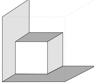
Figure 2: Example of Fichera-type corner domain.
