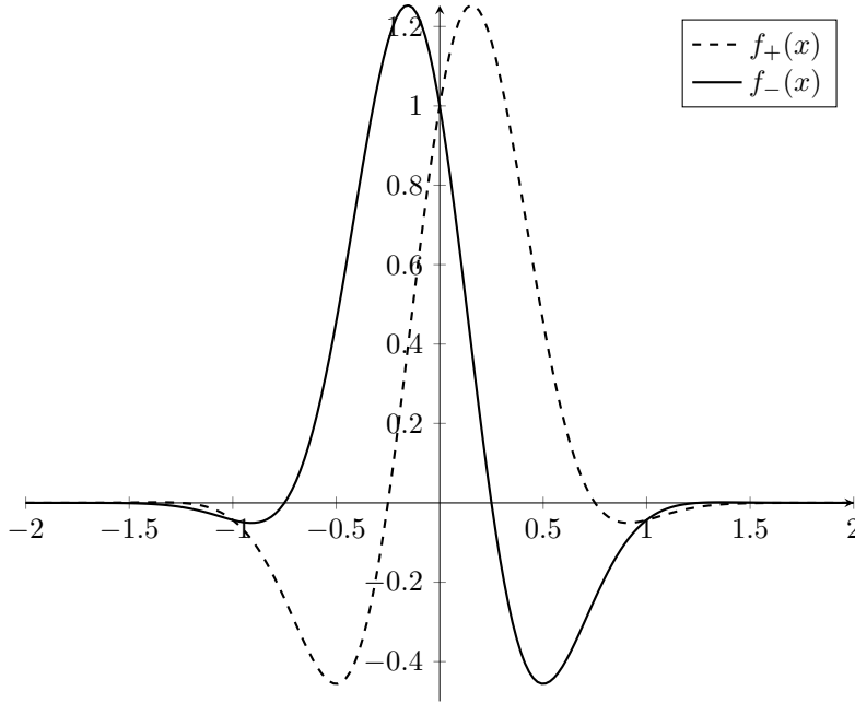
Figure 1: The functions defined in equation (2) with a = 1 .
