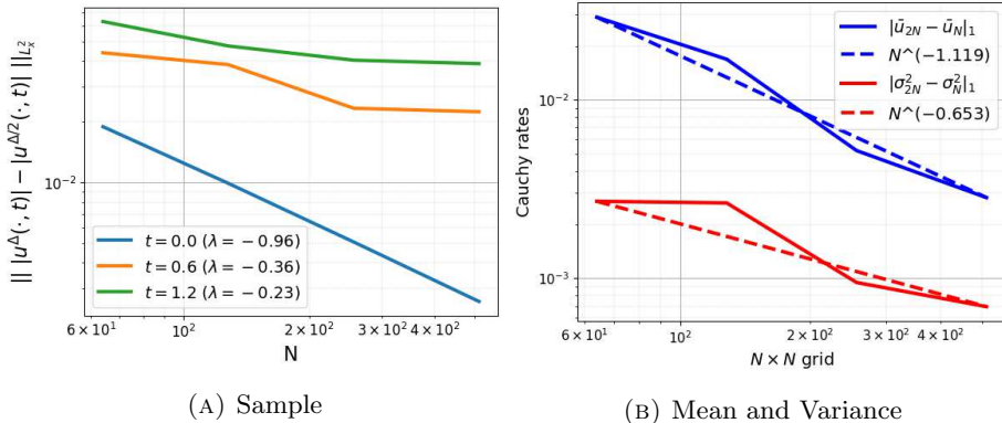
FIGURE 8. Cauchy rates for the norm of the velocity field ( \sqrt{u_1^2 + u_2^2} ) for the sinusoidal vortex sheet. Slope \lambda is determined by a best fit. Left: Sample convergence rates at three different times t = 0, 0.6, 1.2 . Right: Convergence of mean and variance at T = 1.2
