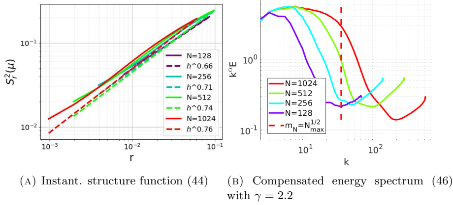
FIGURE 9. The structure function and compensated energy spectrum for the sinusoidal vortex sheet at time T = 1.2
