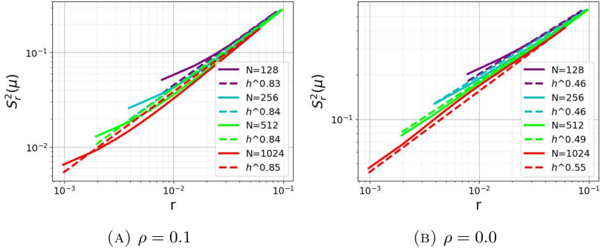
FIGURE 3. Instantaneous structure function (44) vs correlation length r for different resolutions ( N \sim \Delta^{-1} ) for different values of smoothness parameter \rho , at t = 0.4
