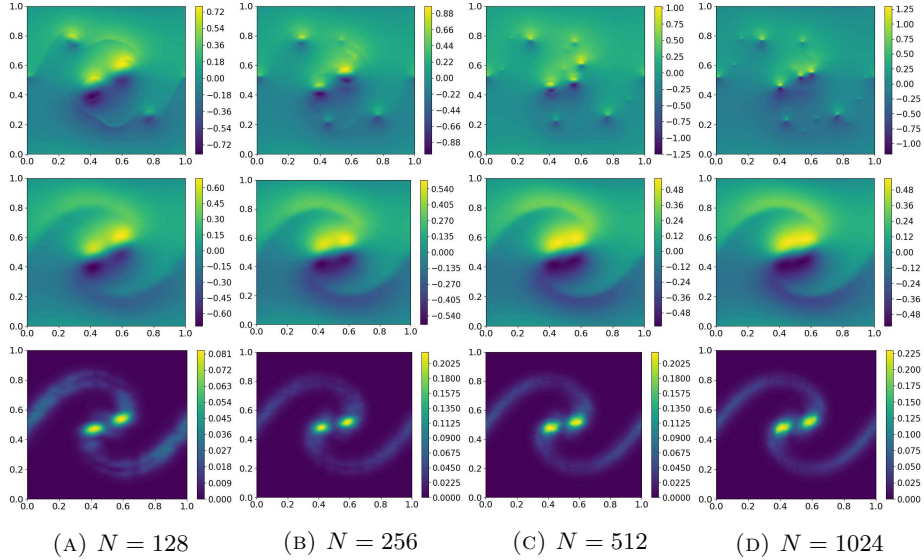
FIGURE 7. Results at time T = 1.2 for the horizontal velocity u_1 of the sinusoidal vortex sheet, at different resolutions. Top Row: Sample; Middle Row: Mean; Bottom Row: Variance.
