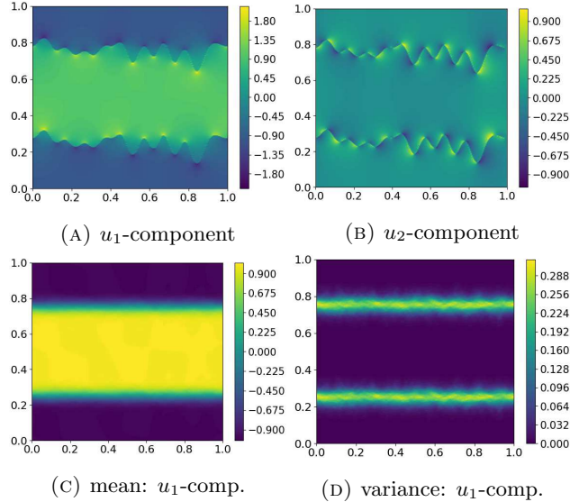
FIGURE 2. Initial data for the perturbed discontinuous flat vortex sheet ( \rho = 0 ), samples for u_{1,2} , and mean and variance of u_1
