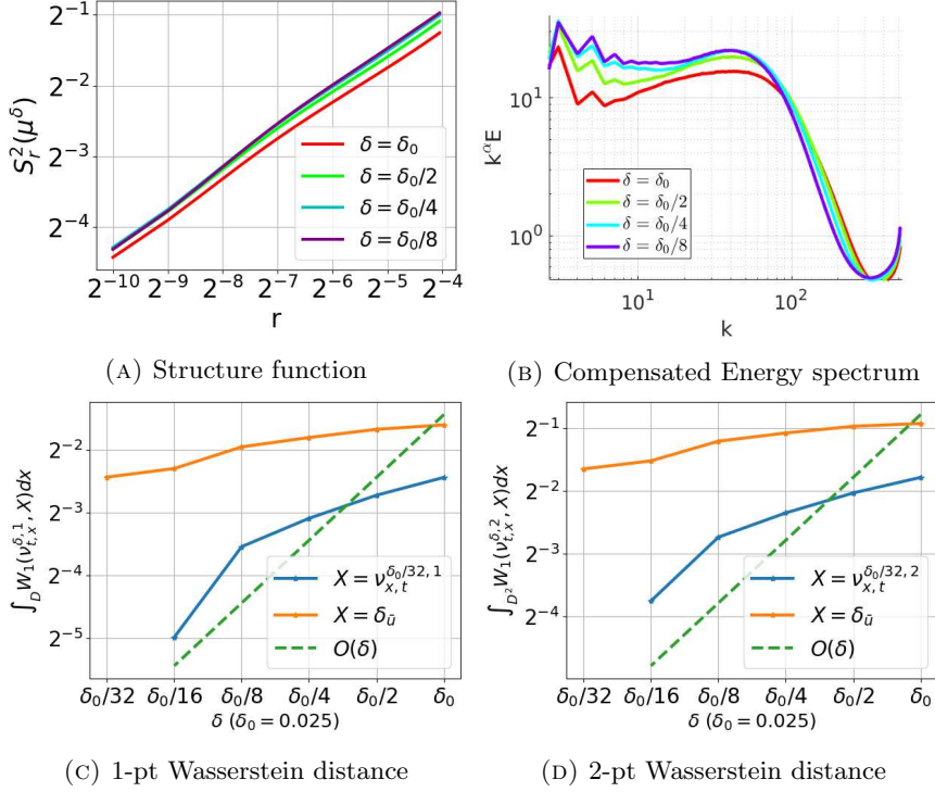
FIGURE 15. Stability of the flat vortex sheet (42) to amplitude of perturbations \delta . Top Row: Instantaneous structure function (44) (Left) and Compensated energy spectrum (39) with \gamma = 2 (Right) at time T = 0.4 for different values of \delta . Bottom Row: Wasserstein distances with respect to the stationary solution (orange) and reference statistical solution (blue) for the 1-point (Left) and 2-point (Right) correlation marginals.
