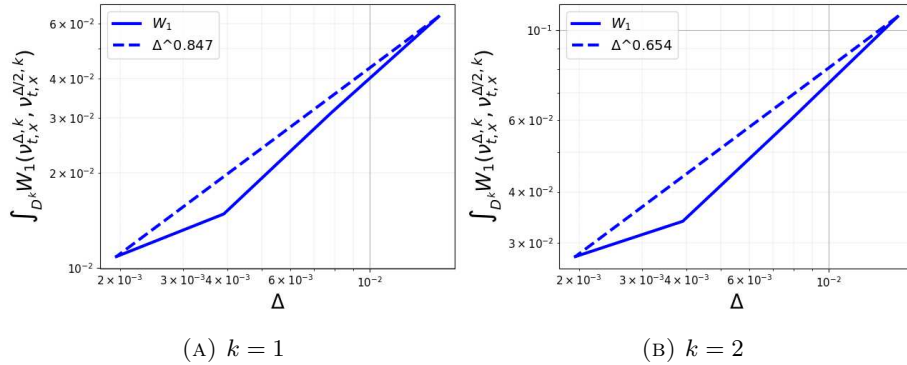
FIGURE 10. The metrics \int_{D^k} W_1(\nu_{t,x}^{\Delta,k}, \nu_{t,x}^{\Delta/2,k}) dx for the one- and two-point correlation marginals for the sinusoidal vortex sheet at time t = 1.2
