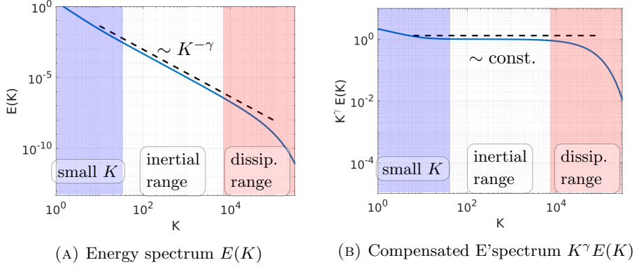
FIGURE 1. Typical energy spectrum for turbulent flows
