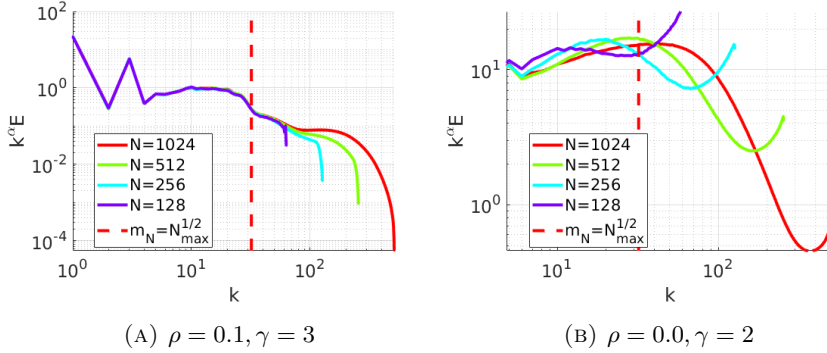
FIGURE 4. The instantaneous compensated energy spectrum \mathcal{C}_{\gamma,t}^{\Delta}(\mu_t; K) (46) for the flat vortex sheet, at time t = 0.4 . Note different values of \gamma for the smooth and discontinuous vortex sheets
