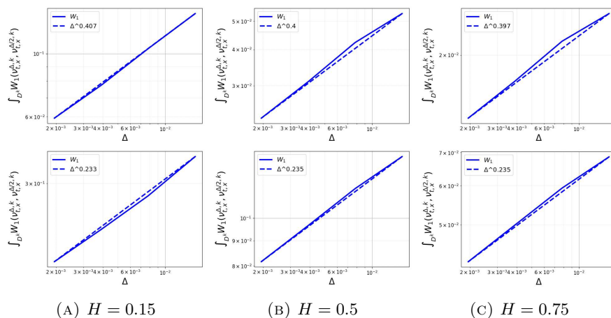
FIGURE 13. Wasserstein distances \int_{D^k} W_1(\nu_{t,x}^{\Delta,k}, \nu_{t,x}^{\Delta/2,k}) dx for k = 1 (Top Row) and k = 2 (Bottom Row) for Fractional Brownian motion initial data with three different Hurst indices at time t = 1 .
