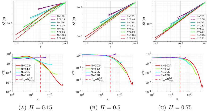
FIGURE 12. Instantaneous structure function (44) (Top Row) and Compensated energy spectrum (46) (Bottom Row) for Fractional Brownian motion initial data with three different Hurst indices at time T = 1 . The compensated energy spectrum (46) is computed with \gamma = 1.3 ( H = 0.15 ), \gamma = 2.0 ( H = 0.5 ) and \gamma = 2.5 ( H = 0.75 )
