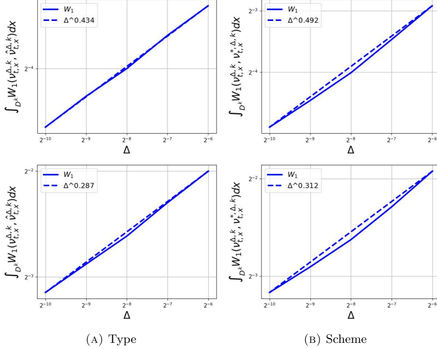
FIGURE 14. Stability of the flat vortex sheet (42) to perturbations. For k = 1 (Top Row) and k = 2 (Bottom Row) and at time t = 0.4 , we plot Left Column: Distance \int_{D^k} W_1(\nu_{t,x}^{\Delta,k}, \hat{\nu}_{t,x}^{\Delta,k}) dx with \hat{\nu} the correlation marginal corresponding to a Normally distributed initial measure in (42). Right Column: Distance \int_{D^k} W_1(\nu_{t,x}^{\Delta,k}, \nu_{t,x}^{*,\Delta,k}) dx with \nu^* the correlation marginal computed with the finite difference projection method.
