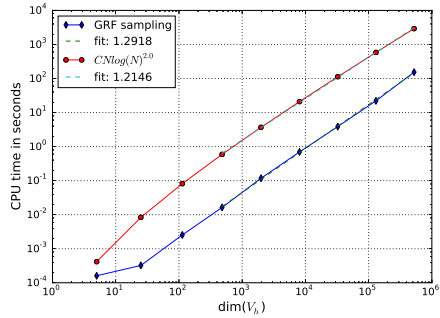
(b) CPU time per sample versus N_h = \dim(V_h) for \widetilde{\mathcal{Z}}_{K,h}^\beta for \beta = 0.75
