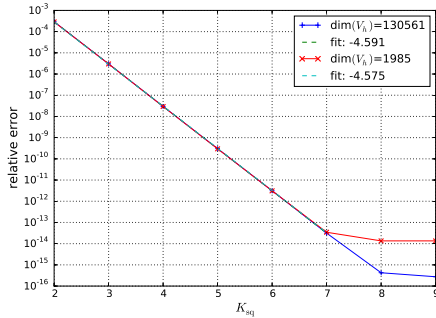
(a) Relative approximation error of \sqrt{\mathbf{M}}\mathbf{y}
