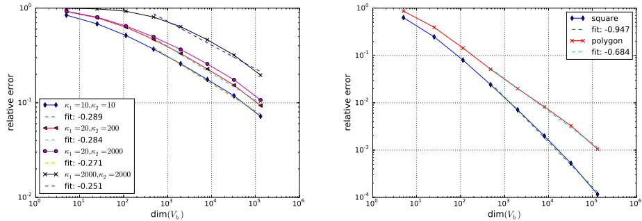
(a) \mathcal{D}_1 = (0, 1)^2 , \beta = 0.75
