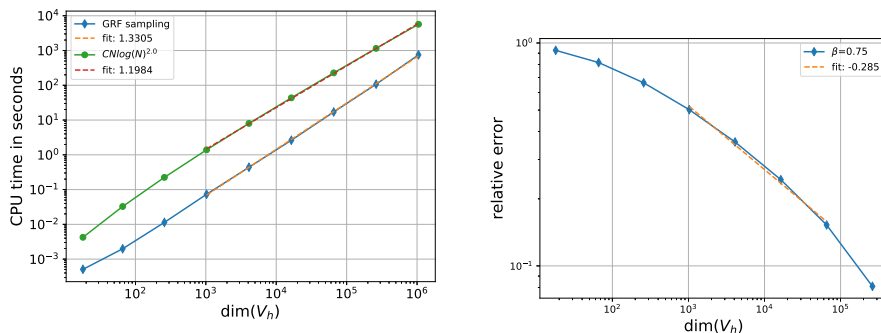
(a) CPU time per sample versus N_h = \dim(V_h) for \tilde{\mathcal{Z}}_{K,h}^\beta with \beta = 0.75 on \mathbb{S}^2 (b) Relative L_2(\Omega; L_2(\mathbb{S}^2)) -error of \tilde{\mathcal{Z}}_{K,h}^\beta for \beta = 0.75 , \kappa_1 = 20 , \kappa_2 = 200
