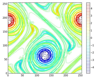
(f) Vorticity at t = 14 , Algorithm 5
