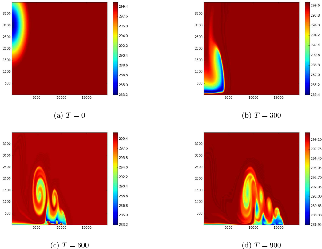
Figure 11: Entropy temperature \theta for test case 5.2.2 in a 2D vertical domain ( y axis represents height)
