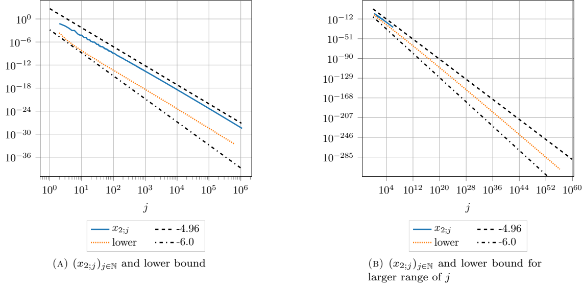
FIGURE 5. Decay of (x_{2;j})_{j \in \mathbb{N}} in (5.12) for \theta = 0.25 and r = 3 . The lower bound is given in Lemma 5.8. For any \delta > 0 there exists C > 0 such that x_{2;j} \leq Cj^{-2r+\delta} = Cj^{-6+\delta} for all j \in \mathbb{N} . In the preasymptotic range a worse rate is observed.
