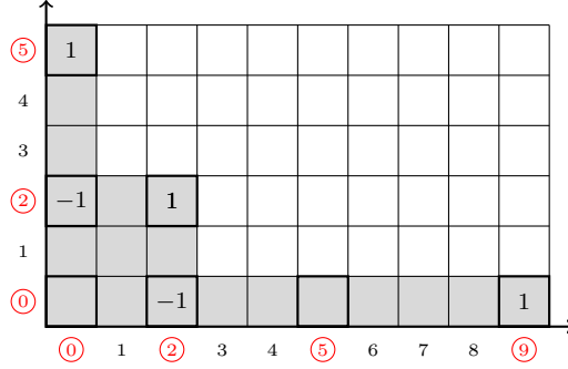
FIGURE 1. The sketch shows a set \Lambda \subseteq \mathbb{N}_0^2 of multiindices corresponding to the grey squares. Equation (2.10) is satisfied for some set \mathfrak{J} = \{0, 2, 5, 9, \dots\} . By Lemma 2.6, \varsigma_{\Lambda, \nu} \neq 0 can only be true if \nu_j \in \mathfrak{J} for all j \in \mathbb{N} . The numbers in the squares show the values of \varsigma_{\Lambda, \nu} for each \nu \in \Lambda with \varsigma_{\Lambda, \nu} \neq 0 .
