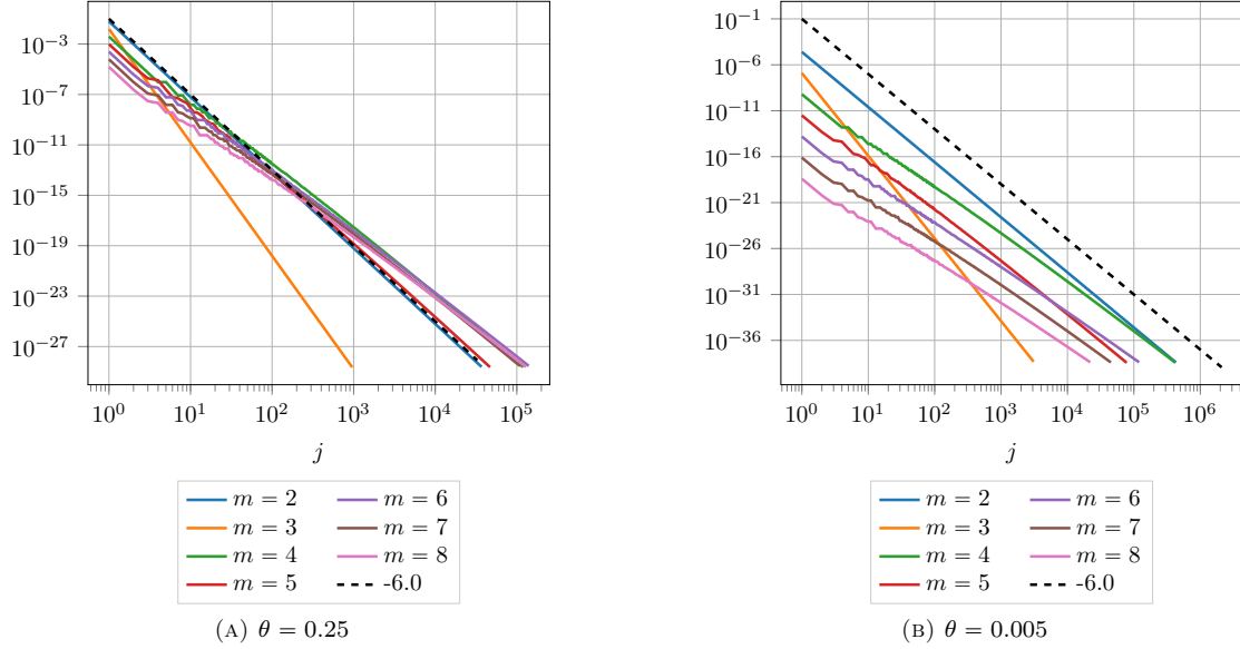
FIGURE 4. Decay of (x_{2;m;j})_{j \in \mathbb{N}} in (5.13) for r = 3 and different values of \theta . For any \delta > 0 and all m \geq 2 there exists C > 0 such that x_{2;m;j} \leq Cj^{-6+\delta} for all j \in \mathbb{N} .
