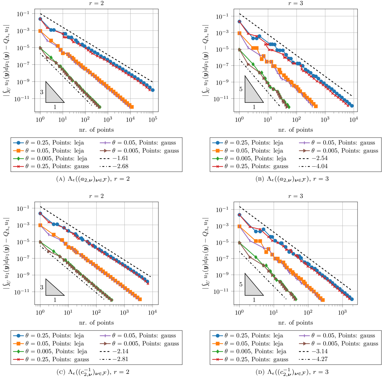
FIGURE 6. Quadrature error |\int_U u_1(\mathbf{y})d\mu_1(\mathbf{y}) - Q_{\Lambda_\epsilon} u_1| for u_1 in (5.25), for different values of r and \theta . The plot shows the absolute error in terms of the number of quadrature points |\text{pts}(\Lambda_\epsilon, \mathcal{X})| (cp. (2.7)).
