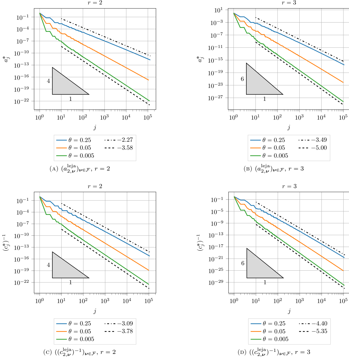
FIGURE 2. Decay of monotonically decreasing rearrangements (a_{2,j}^*)_{j \in \mathbb{N}} and ((c_{2,j}^*)^{-1})_{j \in \mathbb{N}} of (a_{2,\nu}^{\text{leja}})_{\nu \in \mathcal{F}} and ((c_{2,\nu}^{\text{leja}})^{-1})_{\nu \in \mathcal{F}} in (5.6), (5.5). In all cases, the asymptotic algebraic decay rate is 2r - \delta for any \delta > 0 as stated in (5.9).
