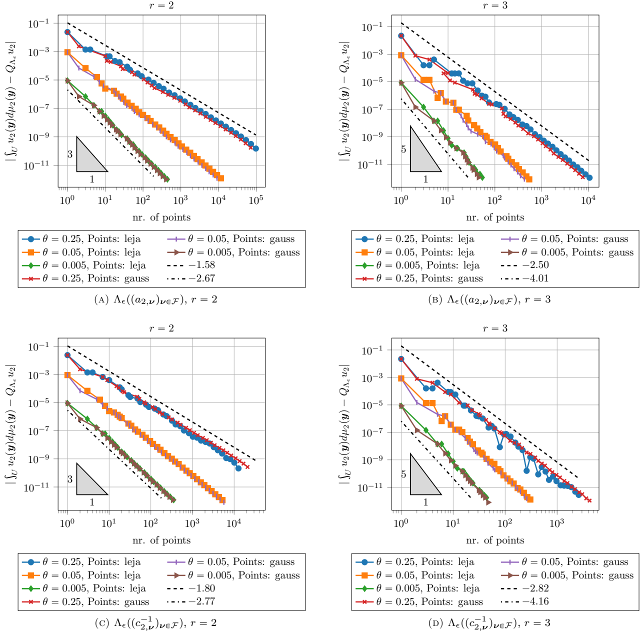
FIGURE 7. Quadrature error |\int_U u_2(\mathbf{y})d\mu_2(\mathbf{y}) - Q_{\Lambda_\epsilon} u_2| for u_2 in (5.25), for different values of r and \theta . The plot shows the absolute error in terms of the number of quadrature points |\text{pts}(\Lambda_\epsilon, \mathcal{X})| (cp. (2.7)).
