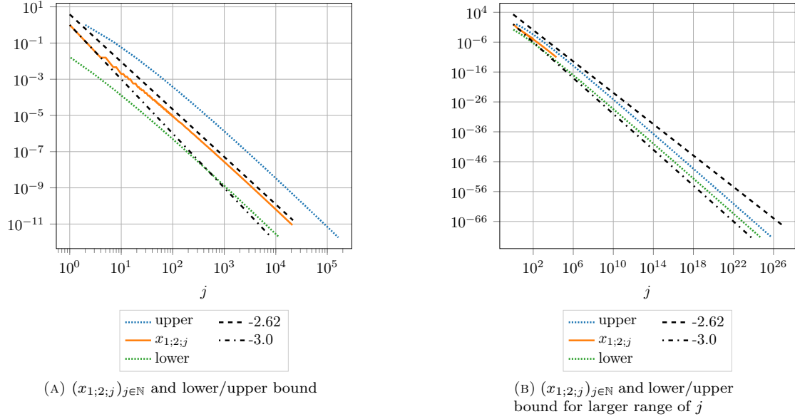
FIGURE 3. Decay of (x_{1;2;j})_{j \in \mathbb{N}} in (5.13) (i.e. m = 2 and k = 1 ), for r = 3 , \theta = 1 . Additionally, the lower and upper bounds of x_{1;2;j} in (5.20) (cp. (5.19)) are depicted. For any \delta > 0 there exists C > 0 such that x_{1;2;j} \leq Cj^{-3+\delta} for all j \in \mathbb{N} . For small j , a worse, preasymptotic rate is observed.
