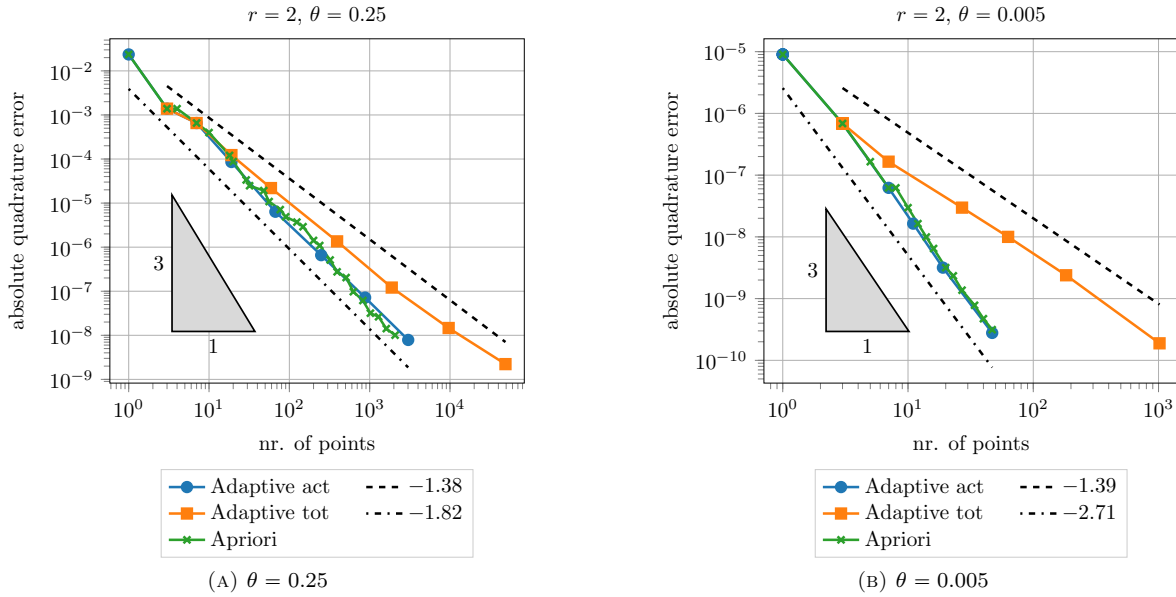
FIGURE 8. Absolute quadrature error for u_2 in (5.26), with r = 2 and different values of \theta . We compare convergence of the adaptive algorithm in Alg. 1 with the Smolyak quadrature based on our apriori choice of index sets. In both cases the same Leja quadrature points (see Sec. 5.1.1) are used.
