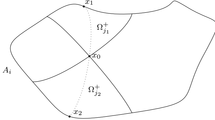
FIGURE 6.1. The level sets of u .
