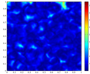
Fig. 22.3. Conditioning of the matrix w_\delta \star \nabla \varepsilon \nabla \varepsilon^T .
