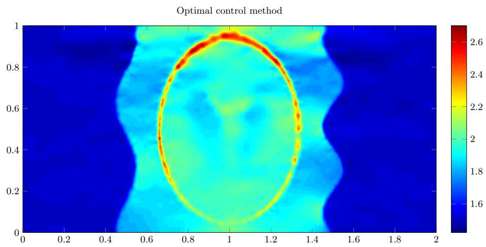
Fig. 15.6. Reconstructed image with 2% measurement noise (each measurement is perturbed by an additive Gaussian random variable with mean zero and standard deviation equal to 2% of the maximal absolute value of the unperturbed measurements).
