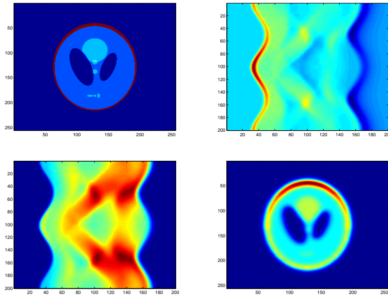
Fig. 13.4. Numerical inversion of attenuated wave equation with K(\omega) given by (13.14) for c_0 = 1 and a = 0.001 . Here N = 256 , N_R = 200 and N_\theta = 200 . Top left: p_0 ; Top right: p_a(y, t) with (y, t) \in \partial\Omega \times ]0, 2[ ; Bottom left: \mathcal{W}[p_a](y, t) with (y, t) \in \partial\Omega \times ]0, 2[ ; Bottom right: \mathcal{R}^* \mathcal{B}[\mathcal{W}[p_a]](x) , x \in \Omega .
