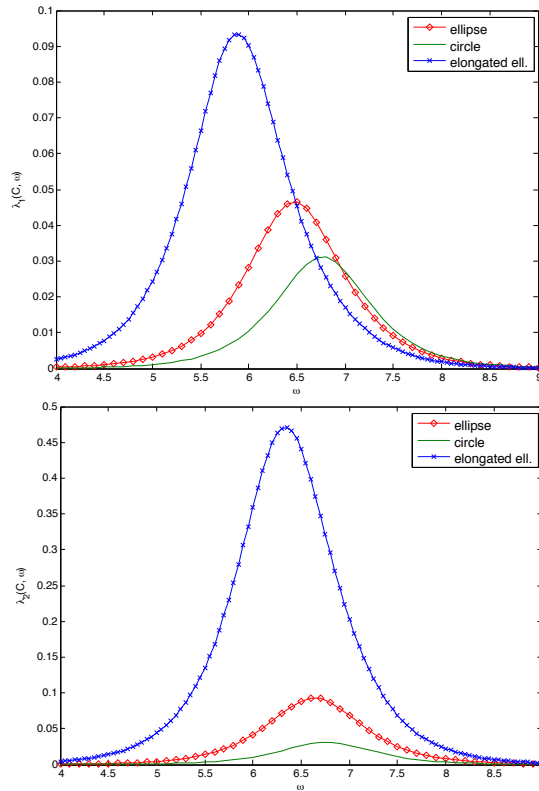
Fig. 23.12. Frequency dependence of the eigenvalues of \mathfrak{S}M for the 3 different cell shapes in Figure 23.11.
