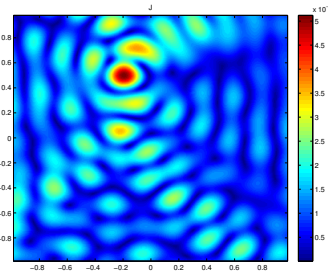
Fig. 25.8. J with 1 illumination.
