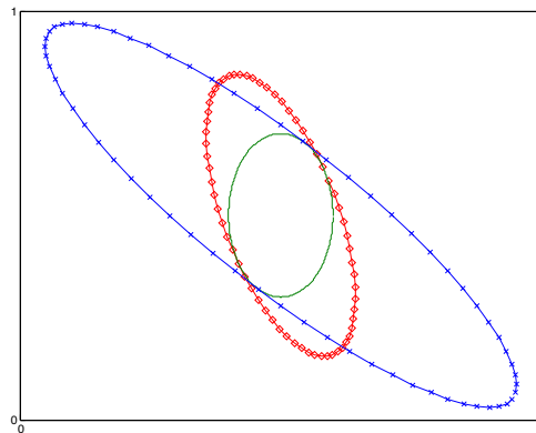
Fig. 23.11. A circle, an ellipse and a very elongated ellipse.
