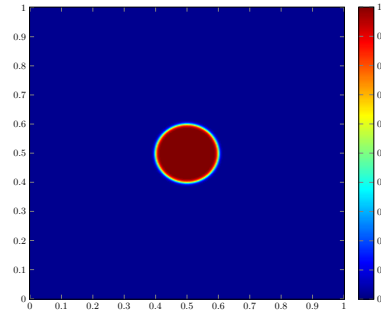
Fig. 22.2. Averaging kernel w_\delta .
