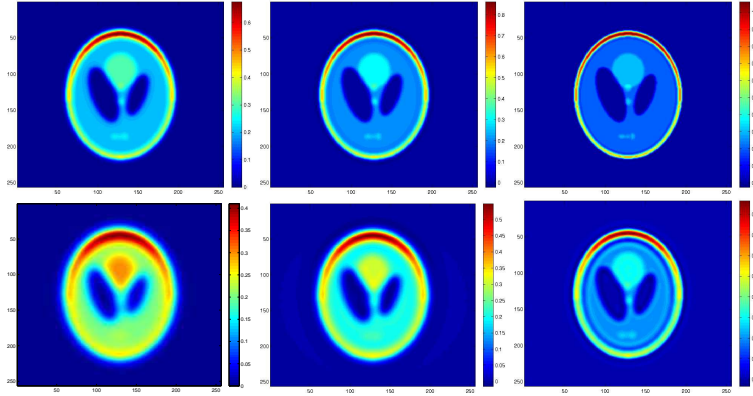
Fig. 13.6. Compensation of acoustic attenuation with formula (13.18): N = 256 , N_R = 200 and N_\theta = 200 . First line: a = 0.0005 ; second line: a = 0.0025 . Left: \tilde{\mathcal{L}}_j^{-1} with j = 0 ; Center: \tilde{\mathcal{L}}_j^{-1} with j = 1 ; Right: \tilde{\mathcal{L}}_j^{-1} with j = 8 .
