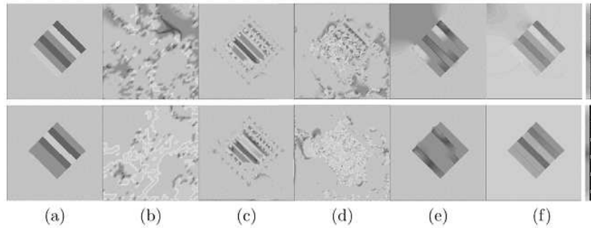
Fig. 21.5. Case 2: Simulation results for \mu (first row) and \eta_\mu (second row) image reconstruction. (a) True images; (c) direct inversion method; (e) hybrid one-step method; (b), (d) and (f) are reconstructed images by the adjoint-based optimization method (21.17) with initial guess of the constant \mu_0 + i\omega\eta_{\mu_0} , (c) and (e), respectively.
