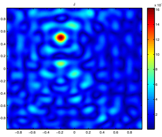
Fig. 25.10. J with 4 illuminations.
