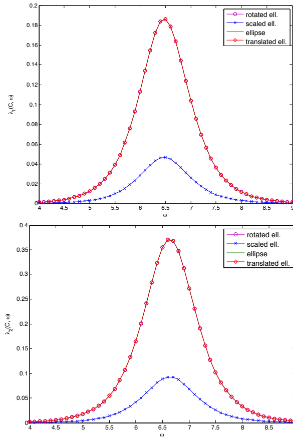
Fig. 23.10. Frequency dependence of the eigenvalues of \Im M for the 4 ellipses in Figure 23.9.
