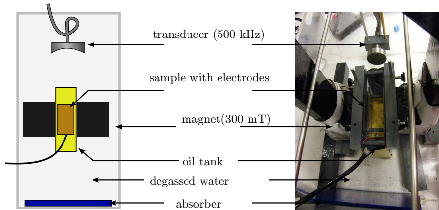
Fig. 15.1. Example of the imaging device. The transducer is emitting ultrasound in a sample placed in a constant magnetic field. An induced electrical current is collected by two electrodes.
