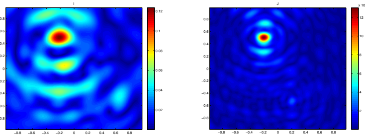
Fig. 25.13. I with 32 illuminations. Fig. 25.14. J with 32 illuminations.
