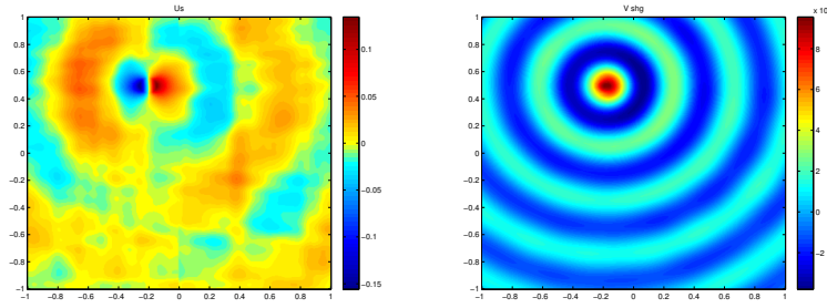
Fig. 25.5. Total scattered field u_s . Fig. 25.6. Second-harmonic field v .
