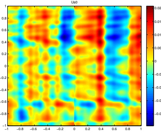
Fig. 25.4. Background field in the absence of a reflector u_s^{(\mu)} .
