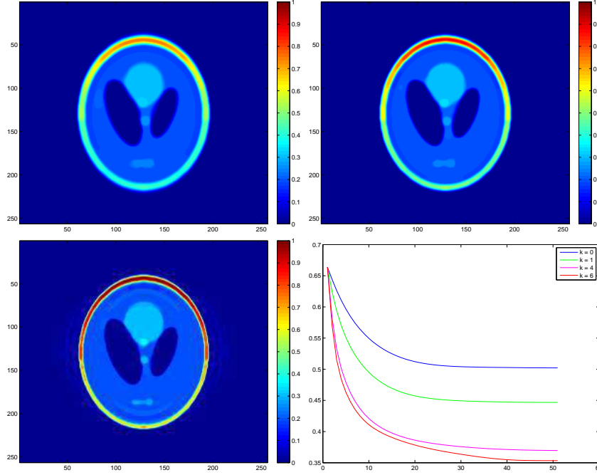
Fig. 13.7. Numerical results using iterative shrinkage-thresholding algorithm with \eta = 0.001 and a = 0.0025 . Left up: f_{50} with k = 0 ; Top right: f_{50} with k = 1 ; Bottom left: f_{50} with k = 6 ; Bottom right: error j \rightarrow \|f_j - p_0\|_{L^2(\Omega)} for different values of k .
