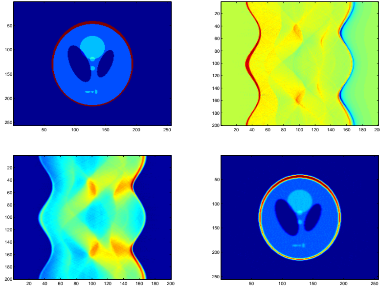
Fig. 13.1. Numerical inversion using (13.8) with N = 256 , N_R = 200 and N_\theta = 200 . Top left: p_0 ; Top right: p(y, t) with (y, t) \in S \times (0, 2) ; Bottom left: \mathcal{R}[p_0](y, t) with (y, t) \in S \times (0, 2) ; Bottom right: \mathcal{R}^* \mathcal{B} \mathcal{R}[p_0] .
