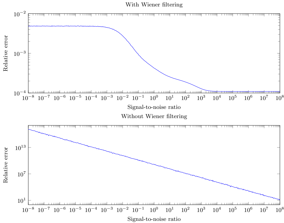
Fig. 15.3. L^2 norm of the relative error \frac{\|\Psi_{y,\xi} - \widetilde{\Psi}_{y,\xi}\|_2}{\|\Sigma\|_2} with respect to the signal-to-noise ratio.
