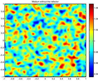
Fig. 25.2. Medium without the reflector (permittivity variations zoomed out).
