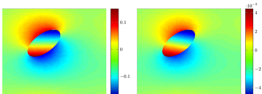
Fig. 23.6. Real and imaginary parts of the cell problem solution w_2 .
