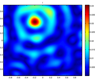
Fig. 25.11. I with 8 illuminations.
