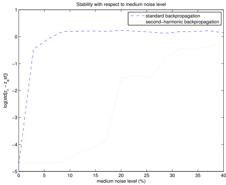
Fig. 25.15. Standard deviation of the localization error with respect to the medium noise level for standard backpropagation (top) and second-harmonic image (bottom).
