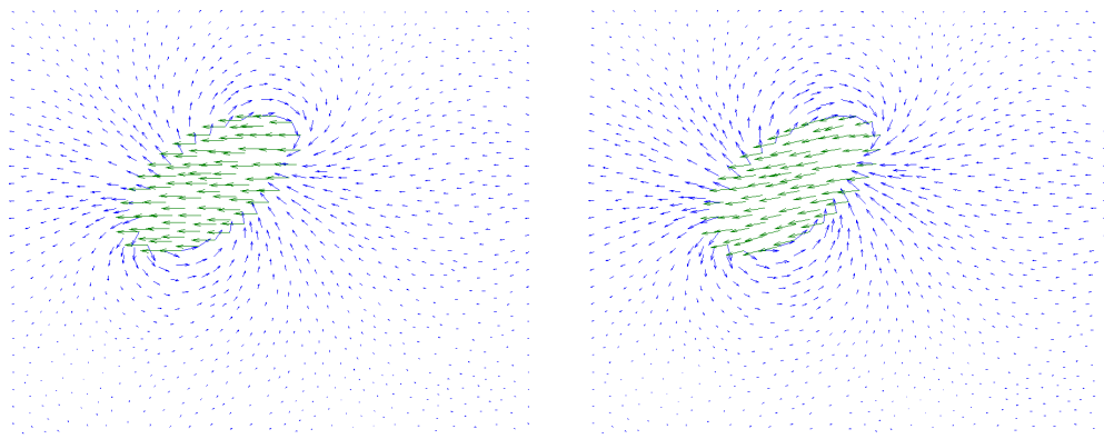
Fig. 23.7. Gradient vector field of the real and imaginary parts of w_1 .
