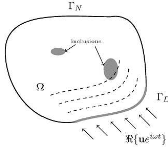
Fig. 21.1. Illustration of the domain and boundary portions.
