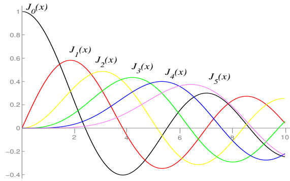
Fig. 2.1. Plots of Bessel functions J_n(x) , n = 0, \dots, 5 .
