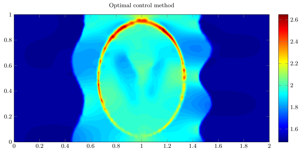
Fig. 15.5. Reconstructed image without measurement noise.
