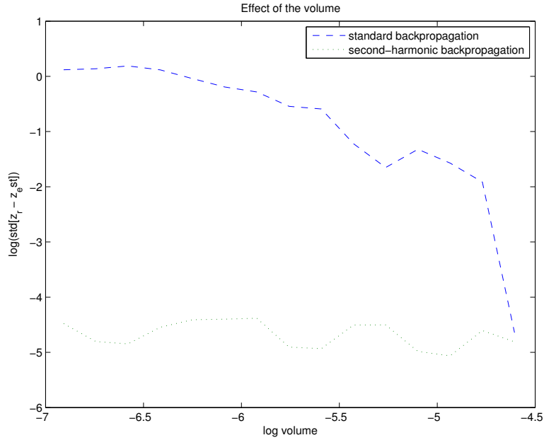
Fig. 25.16. Standard deviation of the localization error with respect to the reflector’s volume (log scale) for standard backpropagation (top) and second-harmonic image (bottom).
