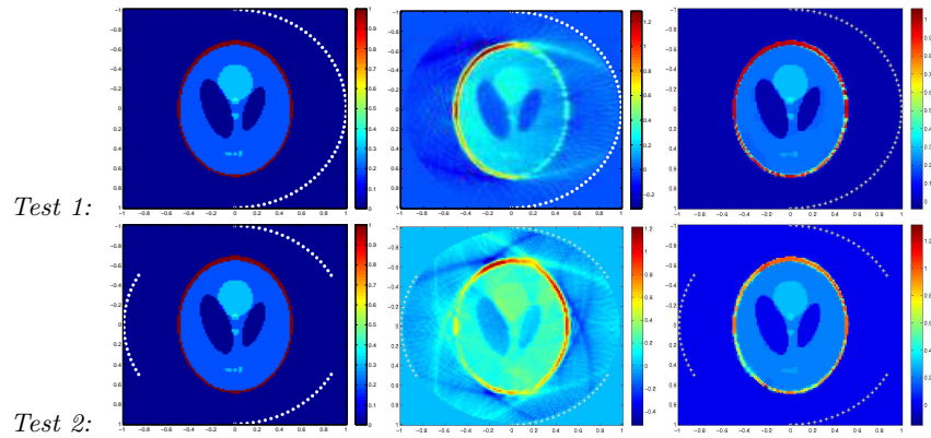
Fig. 13.3. Case of limited angle after 50 iterations, with parameters equal to \eta = 0.01, N = 128, N_R = 128, and N_\theta = 64 . Left: p_0 ; Center: \mathcal{R}^* \mathcal{B} \mathcal{R}[p_0] ; Right: f_{50} .
