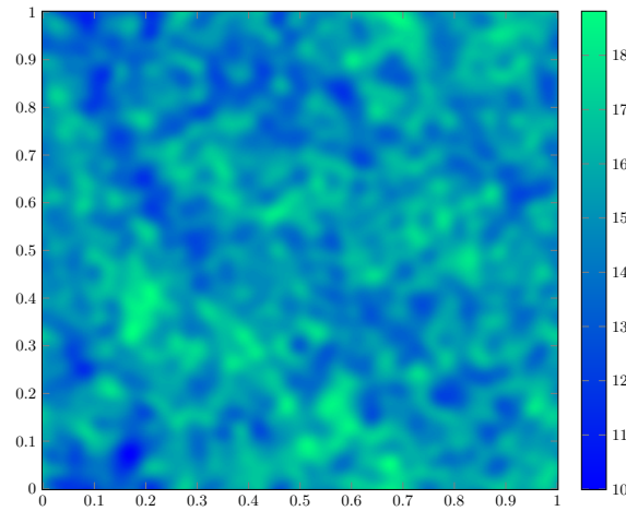
Fig. 22.1. Optical image \varepsilon of the medium.
