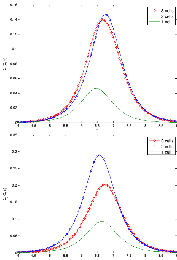
Fig. 23.14. Frequency dependence of the eigenvalues of \Im M in the 3 different cases.
