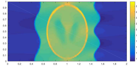
Fig. 16.2. Conductivity reconstructed by the optimal control method after 50 iterations.
