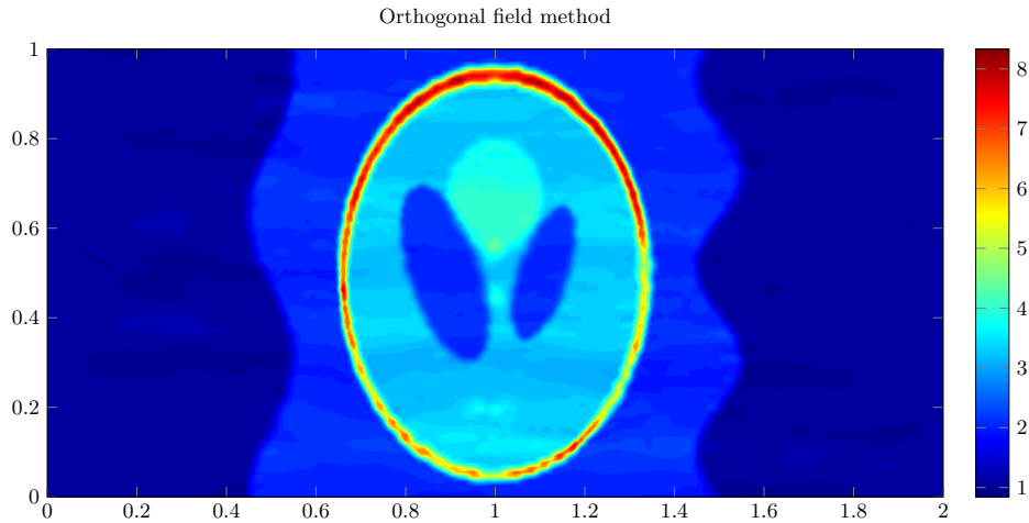
Fig. 15.9. Reconstructed image with 2% measurement noise.
