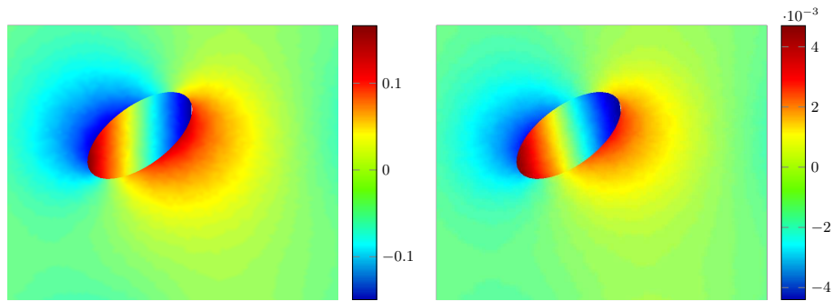
Fig. 23.5. Real and imaginary parts of the cell problem solution w_1 .
