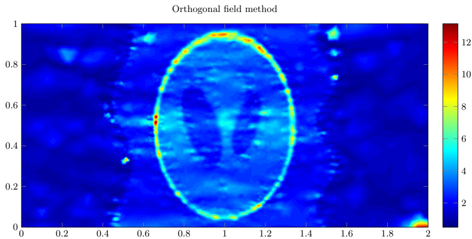
Fig. 15.10. Reconstructed image with 20% measurement noise.
