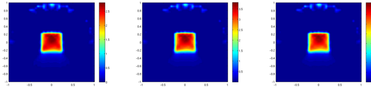
Fig. 19.3. Reconstruction after (from left to right) one, two, and three iterations with \eta = 0.02 , q_i = 3 and \Omega_i = (-0.25, 0.25)^2 , and the measurements N_u are for 50 sources on the unit circle and for r \in (0, 2) .
