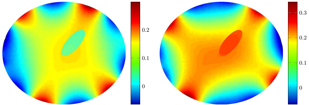
Fig. 23.2. Real and imaginary parts of the potential u outside and inside the cell.
