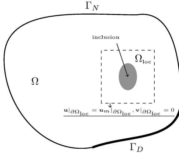
Fig. 21.2. Illustration of the localization of the small anomaly in certain subdomain.
