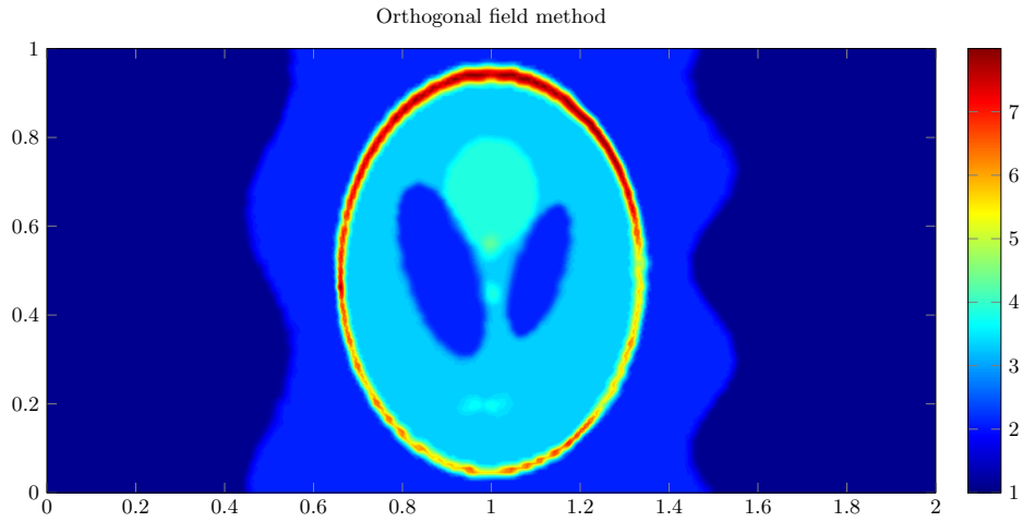
Fig. 15.8. Reconstructed image without measurement noise.
