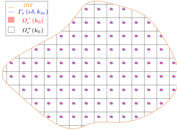
Fig. 23.4. Schematic illustration of the periodic medium \Omega .
