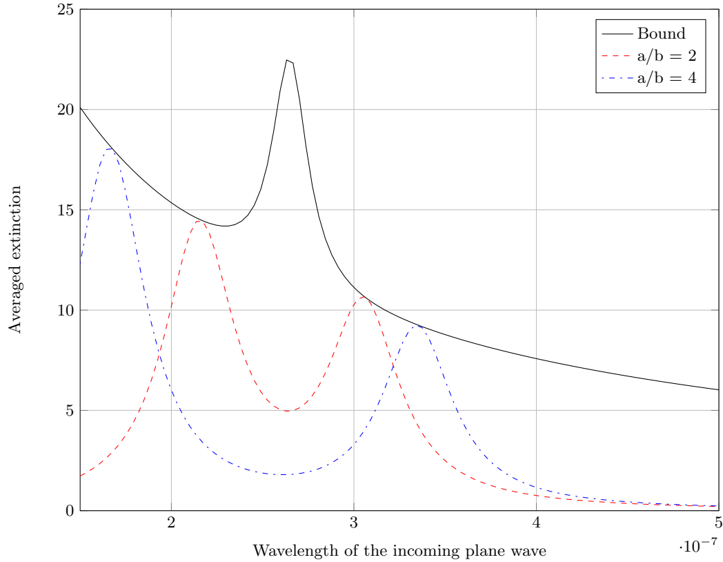
Fig. 24.1. Optimal bound for ellipses.
