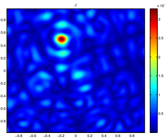
Fig. 25.12. J with 8 illuminations.
