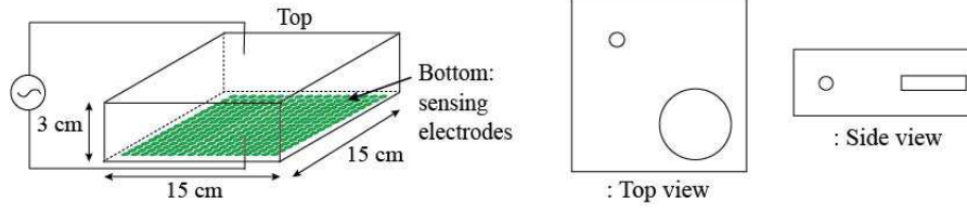
Fig. 20.1. Model for numerical simulations.
