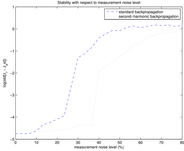
Fig. 25.18. Standard deviation of the localization error with respect to measurement noise level, when averaged over 16 illuminations of angles uniformly distributed between 0 and 2\pi for standard backpropagation (top) and second-harmonic image (bottom).
