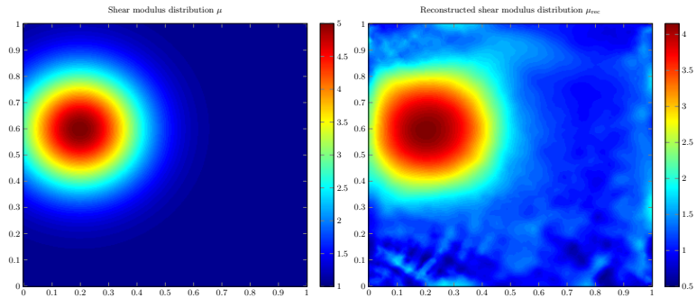
Fig. 22.5. Shear modulus reconstruction.
