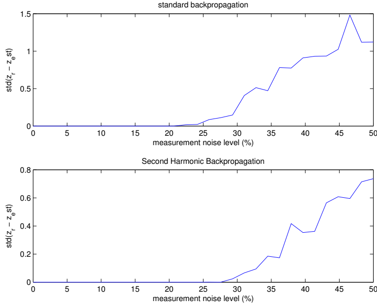
Fig. 25.17. Standard deviation of the localization error with respect to measurement noise level for standard backpropagation (top) and second-harmonic image (bottom).
