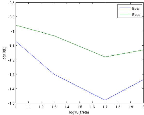
Fig. 19.2. Reconstruction errors E_{val} and E_{pos} as functions of \eta .
