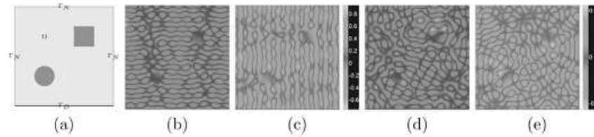
Fig. 21.3. Model 1 and the displacement fields. (a) Model 1; (b) and (c) are real parts of u_1 and u_2 ; (d) and (e) are imaginary parts of them, respectively.
