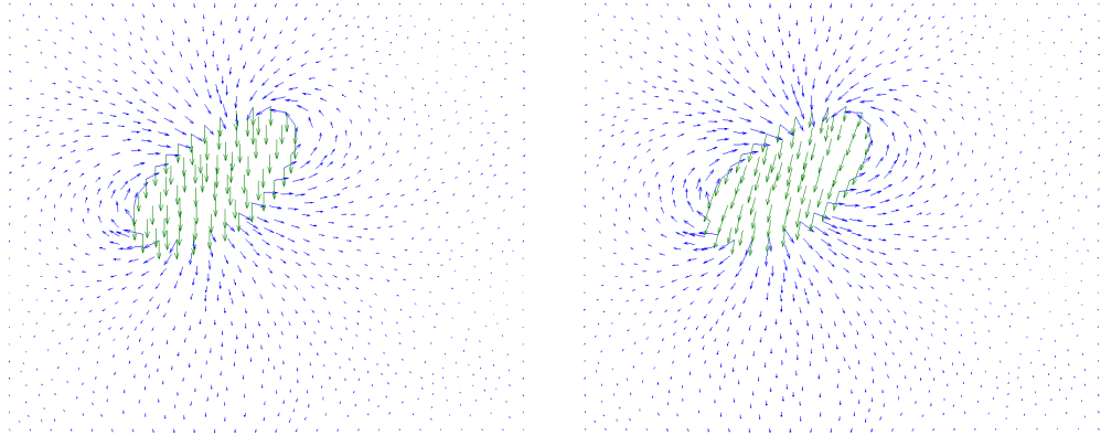
Fig. 23.8. Gradient vector field of the real and imaginary parts of w_2 .
