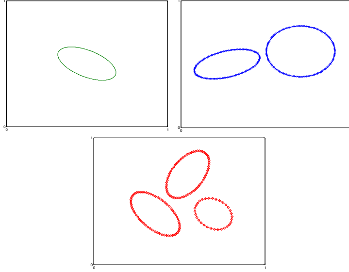
Fig. 23.13. Groups of one, two and three cells.
