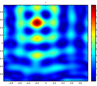
Fig. 25.9. I with 4 illuminations.
