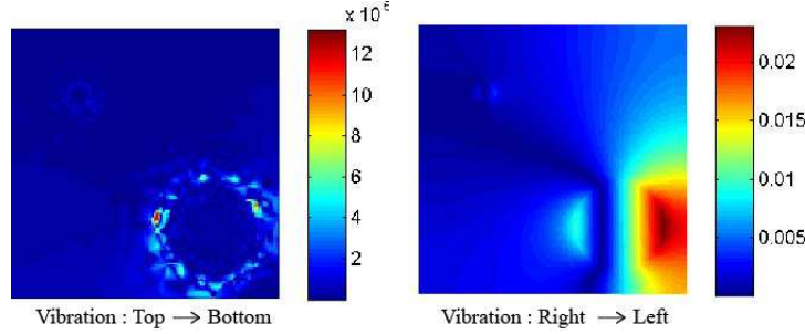
Fig. 20.2. Maps of the voltage difference v_1 on the bottom surface subject to two different mechanical vibrations.
