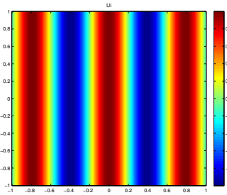
Fig. 25.3. Incoming field U_I .
