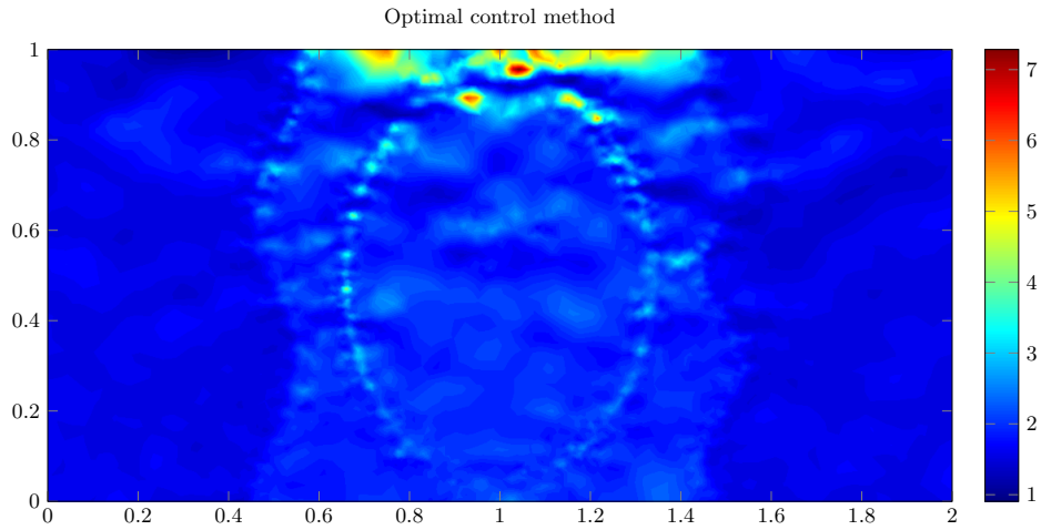
Fig. 15.7. Reconstructed image with 20% measurement noise.
