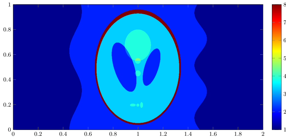
Fig. 15.4. Conductivity map to be reconstructed.
