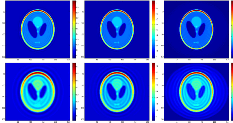
Fig. 13.5. Compensation of acoustic attenuation with SVD regularization: N = 256 , N_R = 200 and N_\theta = 200 . First line: a = 0.0005 ; second line: a = 0.0025 . Left to right: using \mathcal{L}_{1,\gamma}^{-1} respectively with \gamma = 0.01 , \gamma = 0.001 and \gamma = 0.0001 .
