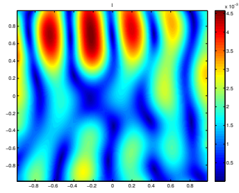
Fig. 25.7. I with 1 illumination.
