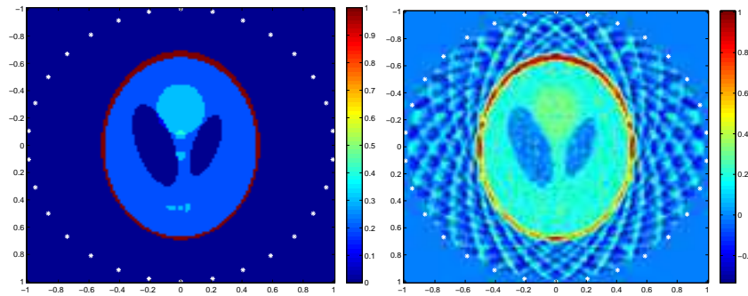
Fig. 13.2. Numerical inversion with truncated (13.8) formula with N = 128 , N_R = 128 , and N_\theta = 30 . Left: p_0 ; Right: \mathcal{R}^* \mathcal{B} \mathcal{R}[p_0] .
