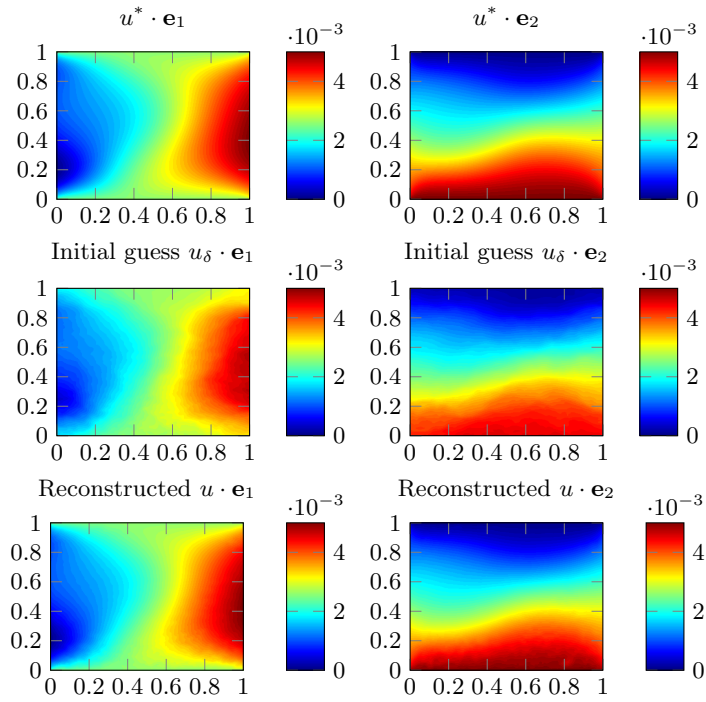
Fig. 22.4. Displacement field and its reconstruction.
