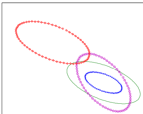
Fig. 23.9. An ellipse translated, rotated and scaled.
