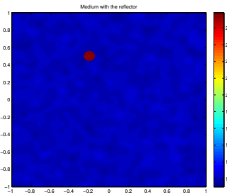
Fig. 25.1. Medium with the reflector.
