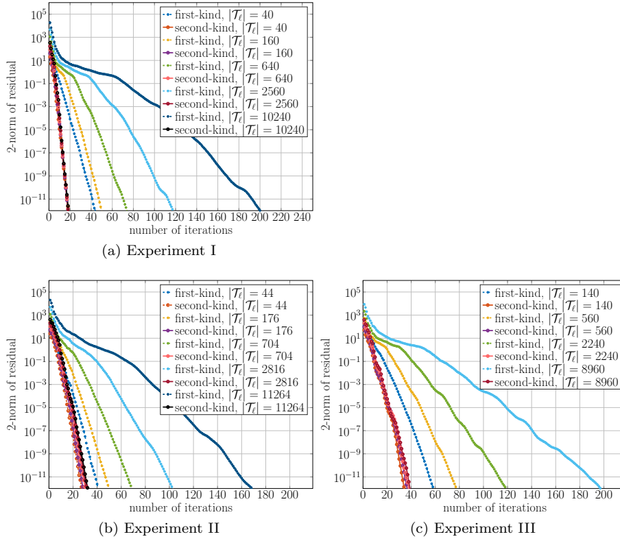
Fig. 6.6: Convergence of GMRES applied to (diagonally rescaled) first- and second-kind Galerkin system.
