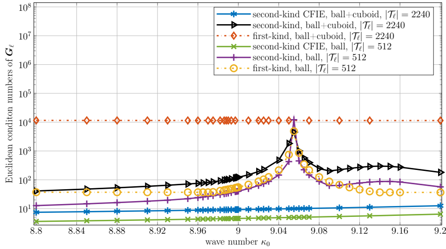
Fig. 6.7: Spurious resonances due to impenetrable objects: condition numbers of the first- and second-kind Galerkin matrix for various wave numbers. In the case of the geometry ball , the scatterer consists of the ball \mathcal{B}_{0.5}(\mathbf{0}) and is impenetrable, while in the case of the geometry ball+cuboid , which refers to the geometry of Experiment III, we set \kappa_0 = \kappa_2 and assume that \Omega_1 is impenetrable as well.
