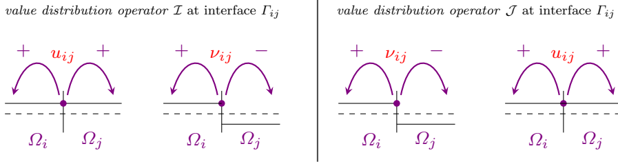
Fig. 3.1: Visualization of the local action of the mappings \mathcal{I} , \mathcal{J} at the interface \Gamma_{ij} acting on an L^2 skeleton function \mathbf{u}_{ij} = (u_{ij}, \nu_{ij}) \in \mathcal{L}_{\bullet}^2(\Sigma) . It is important to note the change of the role of Dirichlet and Neumann data inherent in the mapping \mathcal{J} .
