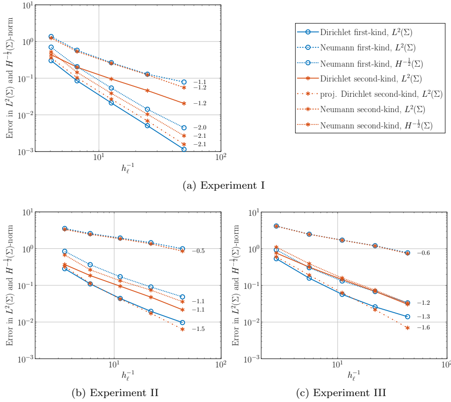
Fig. 6.4: Convergence of the error of (diagonally rescaled) first- and second-kind Galerkin discretization in L^2 - and H^{-\frac{1}{2}} -norm for a sequence of meshes.
