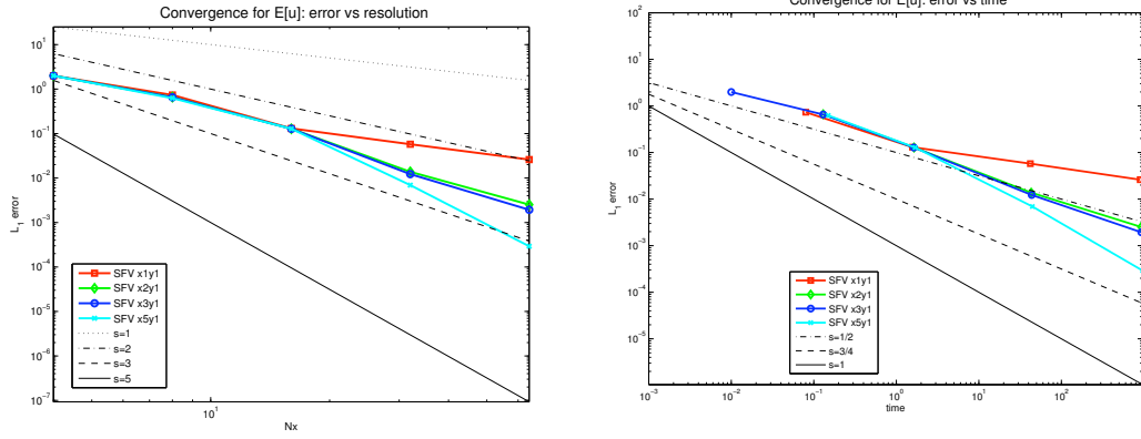
FIGURE 4. Convergence of the stochastic collocation FV method for the solution mean: L^1(\Omega; L^1(\mathbb{R})) -error vs. number of cells in space (left) and vs. CPU time (right)
