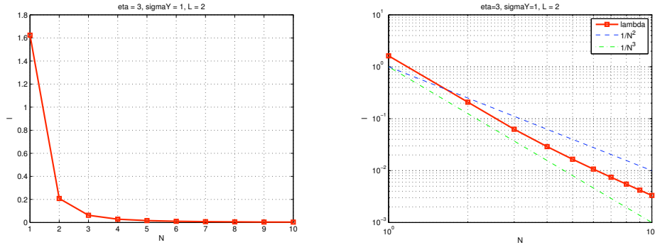
FIGURE 2. Eigenvalues in linear (left) and doubly logarithmic (right) axes
