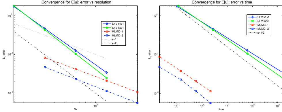
FIGURE 9. Convergence of stochastic collocation FV and MLMC methods at t = 0.5 : L^1(\Omega; L^1(\mathbb{R})) -error vs. number of cells in space (left) and vs. CPU time (right)
