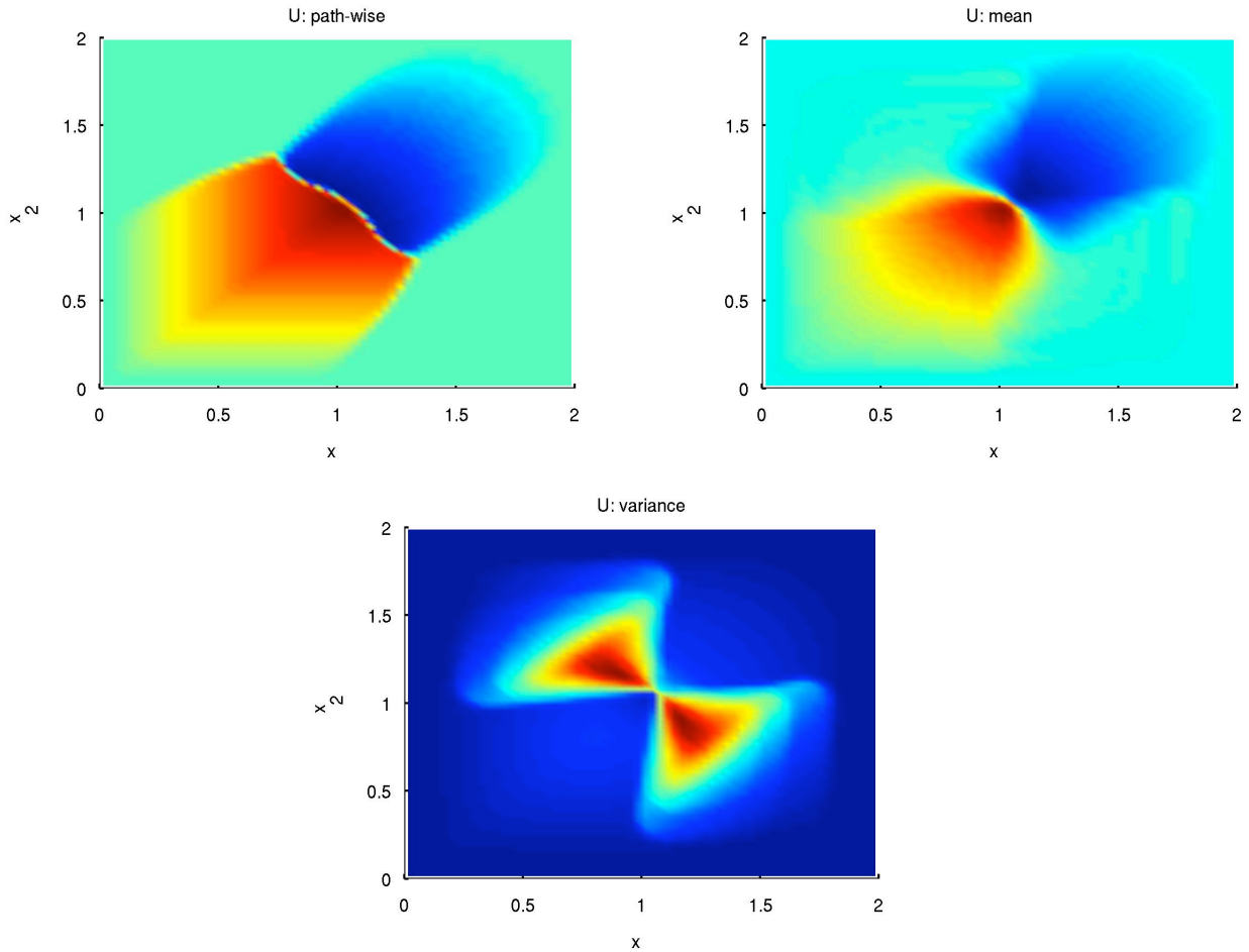
FIGURE 10. Computed sample path (upper left), mean (upper right) and variance (bottom) of the random solution to (6.4)–(6.5) at t = 0.5
