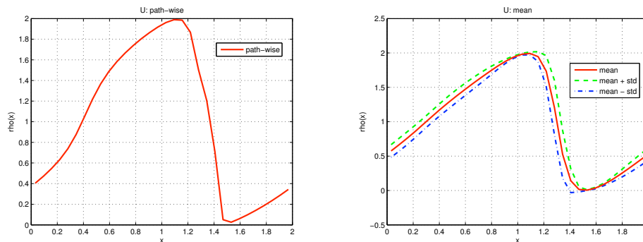
FIGURE 3. Typical sample path of the random solution (left) and mean and mean \pm standard deviation of the random solution (right) at t = 0.2
