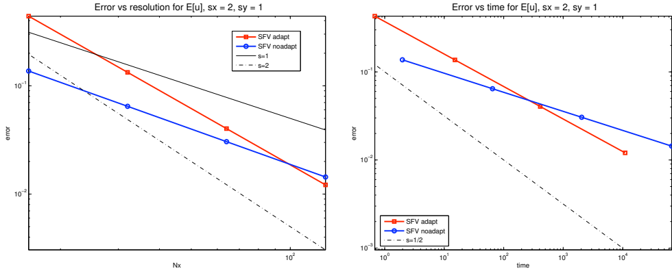
FIGURE 7. Efficiency of the KL-based mesh adaptation at t = 0.5 (shock solution): L^1(\Omega; L^1(\mathbb{R})) -error vs. number of cells in space (left) and vs. CPU time (right)
