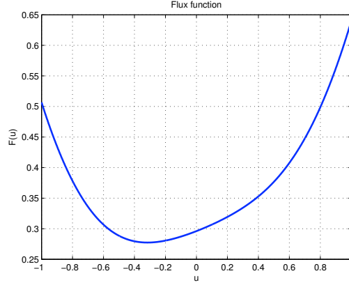
FIGURE 1. Typical realization of the random flux
