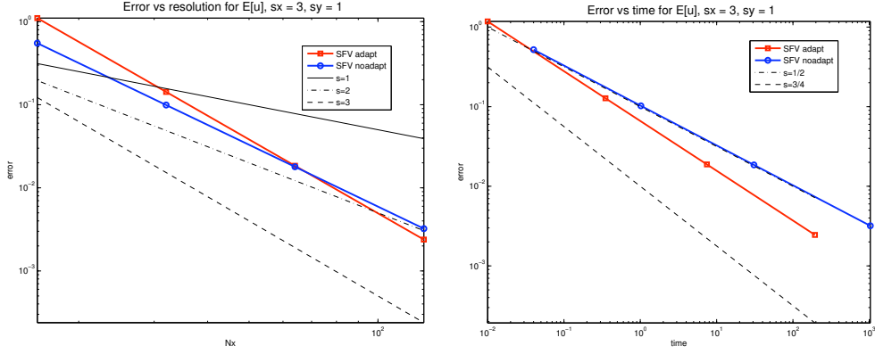
FIGURE 6. Efficiency of the KL-based mesh adaptation at t = 0.1 (smooth solution): L^1(\Omega; L^1(\mathbb{R})) -error vs. number of cells in space (left) and vs. CPU time (right)
