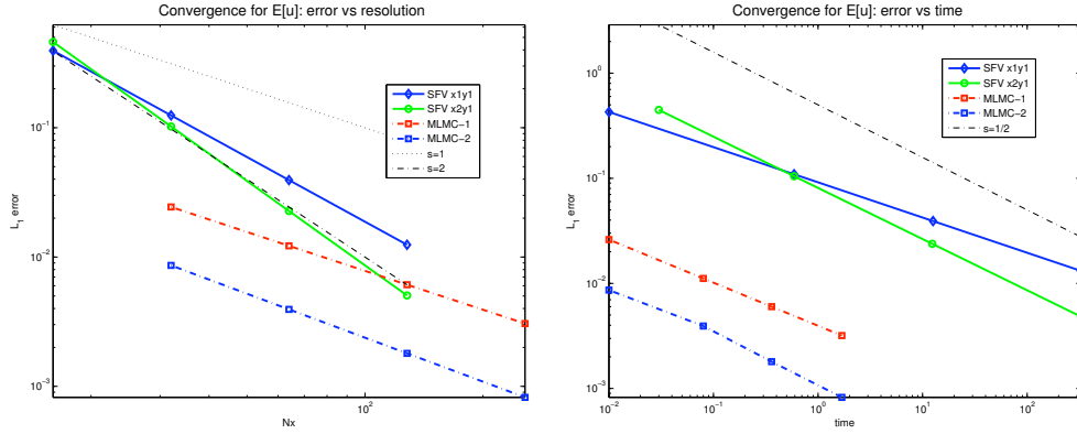
FIGURE 8. Convergence of stochastic collocation FV and MLMC methods at t = 0.1 : L^1(\Omega; L^1(\mathbb{R})) -error vs. number of cells in space (left) and vs. CPU time (right)
