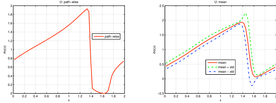
FIGURE 5. Typical sample path of the random solution (left) and mean and mean \pm standard deviation of the random solution (right) at t = 0.5
