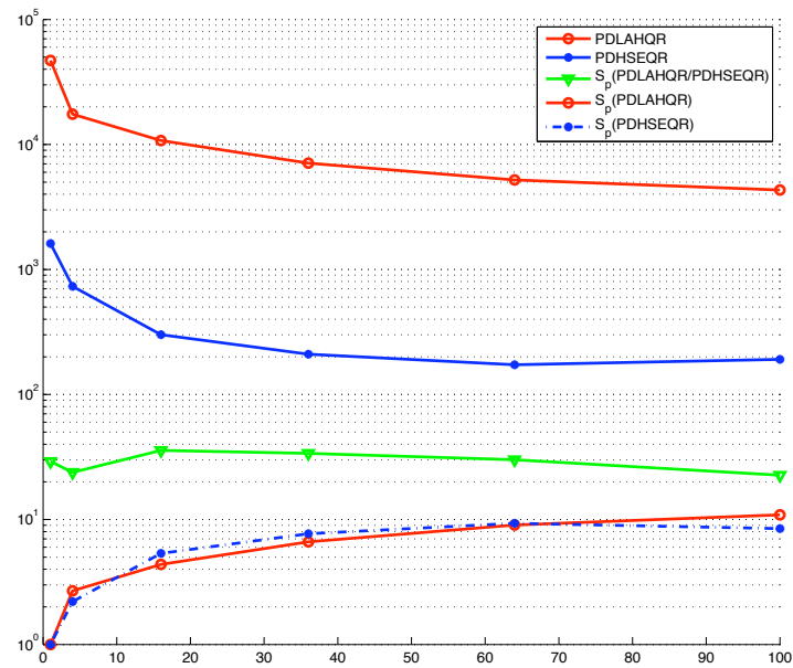
Figure 11: T_p and S_p for PDLAHQR and PDHSEQR applied to CRYG10000 on akka.
