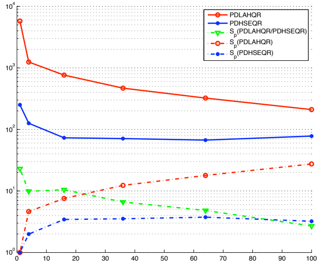
Figure 13: T_p and S_p for PDLAHQR and PDHSEQR applied to OLM5000 on akka . Note that for 4 cores, the time for PDLAHQR is measured for multithreading on one node, which turned out to be faster than using 4 MPI processes inside the node.
