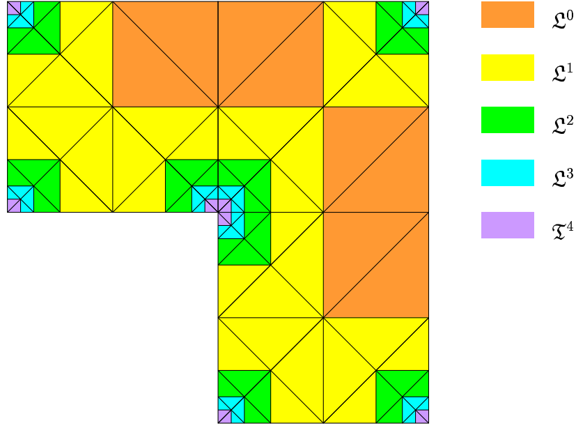
Figure 2: Mesh with triangle elements – case (b).
