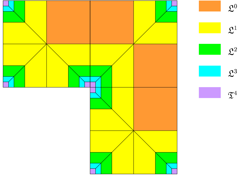
Figure 3: Mesh with Q^1 elements (trapezia) – case (c).
