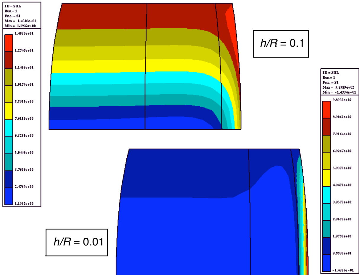
FIGURE 21. Problem 4 - First principal stress distribution at the middle surface of the shell. Shell model 2, Laminated composite case.
