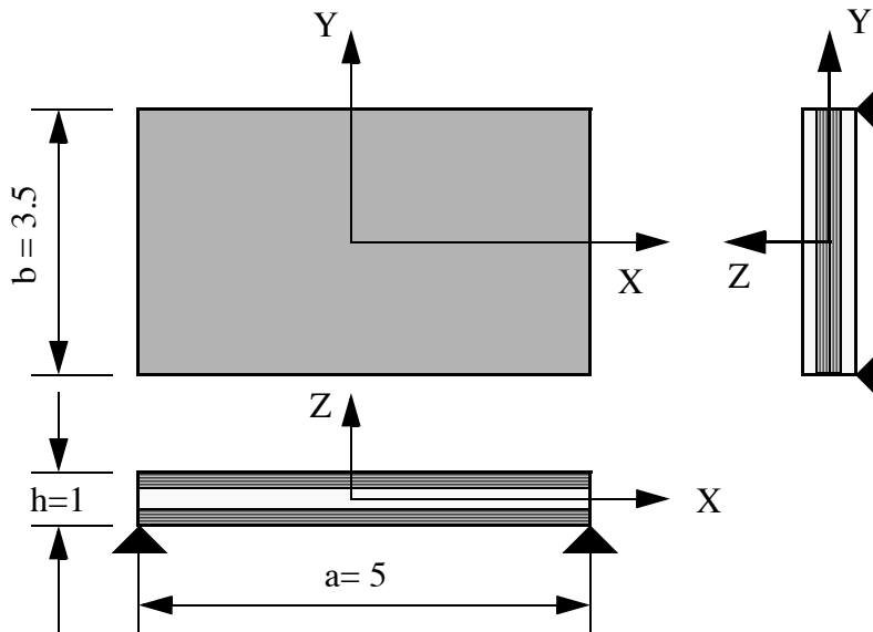
FIGURE 9. Problem 3 - Laminated plate. Notation
