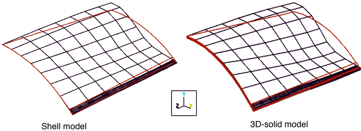
FIGURE 8. Problem 2- Buckling mode shape
