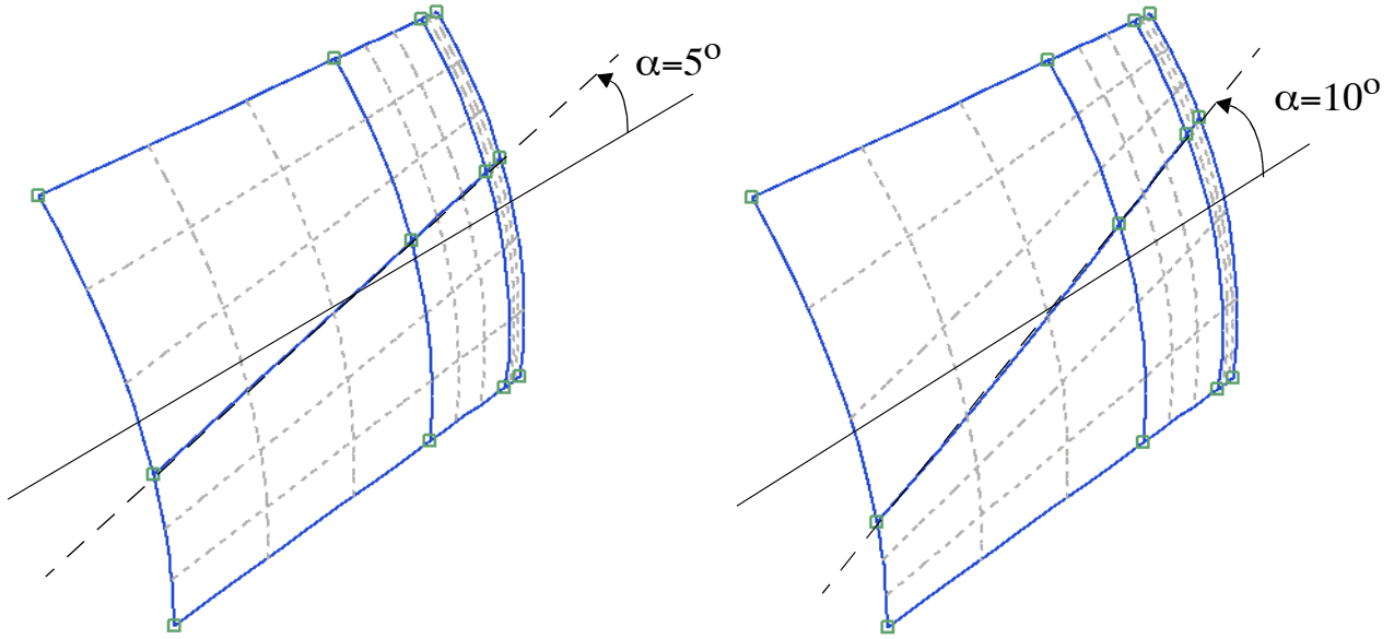
FIGURE 22. Problem 5 - Distorted finite element mesh, 6 elements
