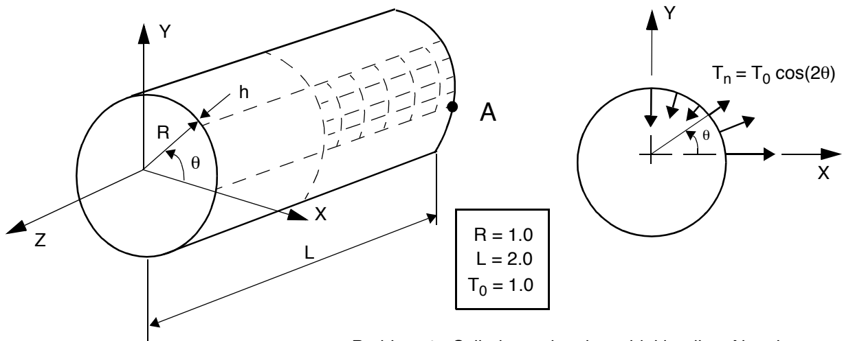
FIGURE 12. Problem 4 - Cylinder under sinusoidal loading. Notation.
