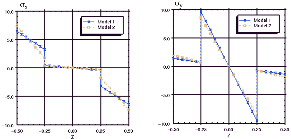
FIGURE 11. Problem 3 - Through-thickness stress distributions \sigma_x(0,0,z) and \sigma_y(0,0,z) for shell models 1 and 2.
