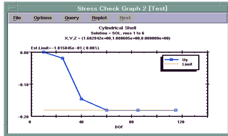
FIGURE 5. Problem 1 - Convergence plot of U_y for the shell model.
