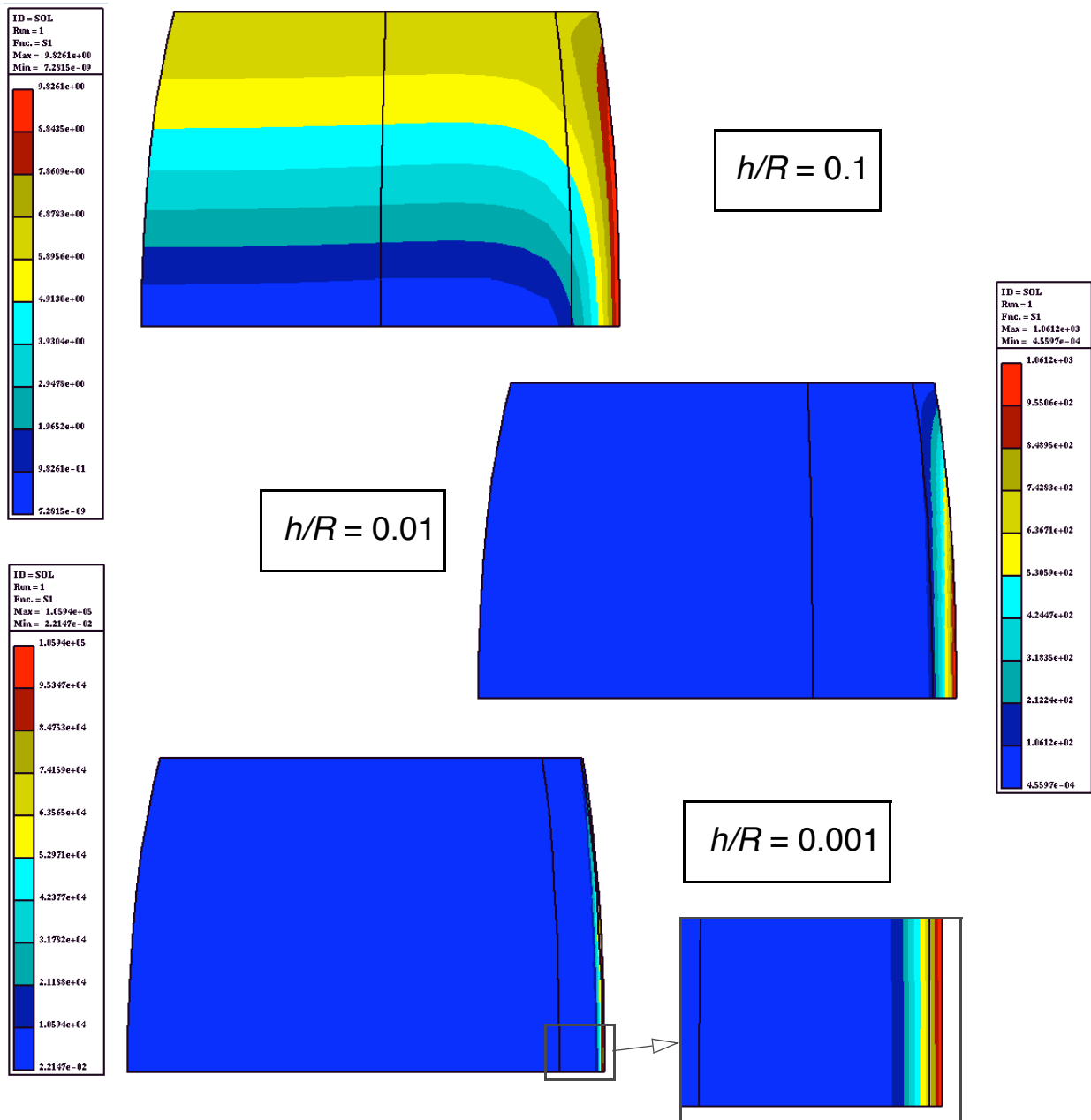
FIGURE 18. Problem 4 - First principal stress distribution at the middle surface of the shell. Shell model 1, Laminated composite case.
