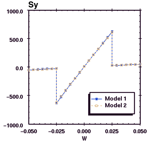
FIGURE 20. Problem 4 - Through-thickness normal stress distribution at point A. Shell models 1 and 2, laminated composite case.
