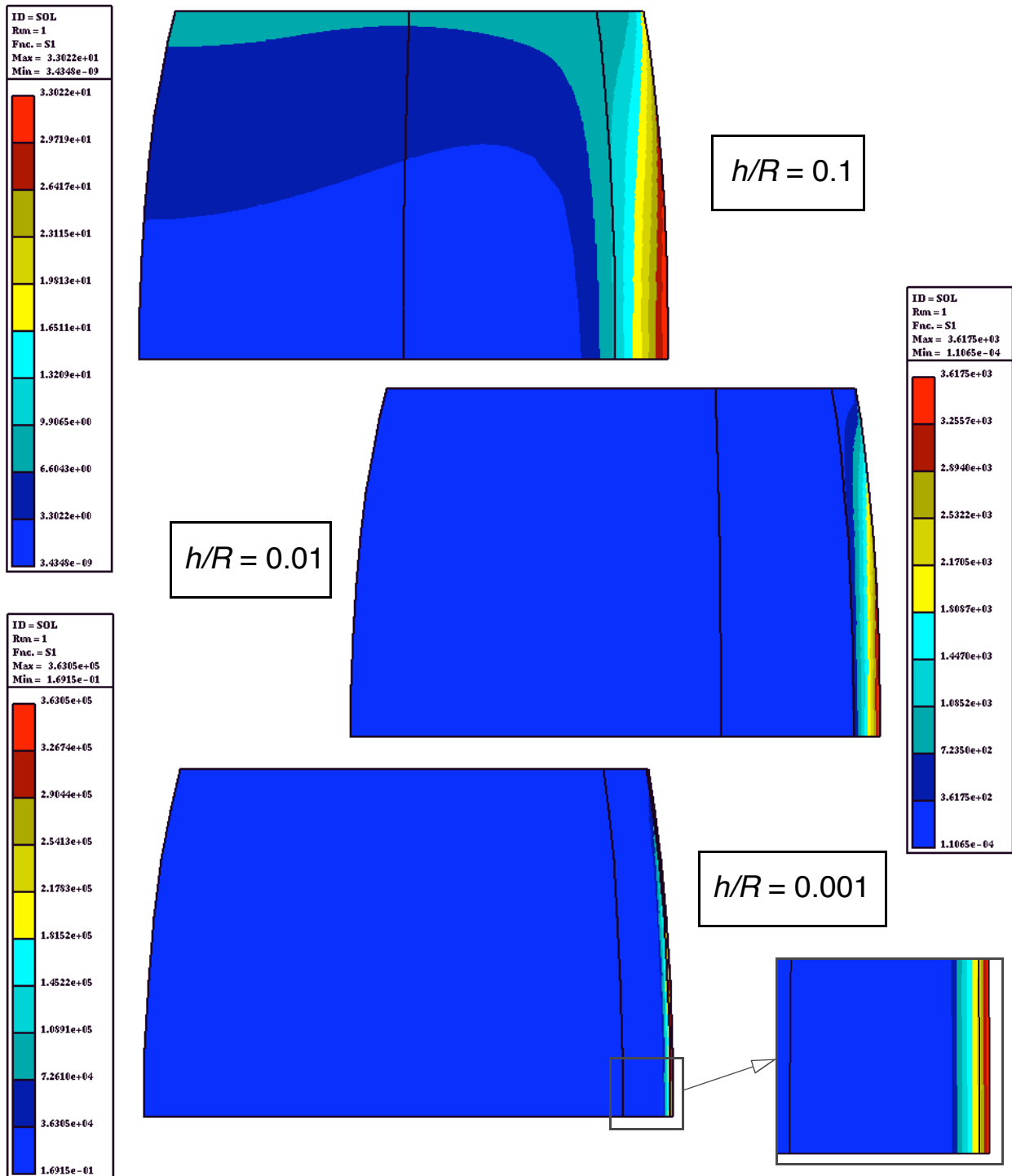
FIGURE 16. Problem 4 - First principal stress distribution at the middle surface of the shell. Shell model 1, isotropic case.
