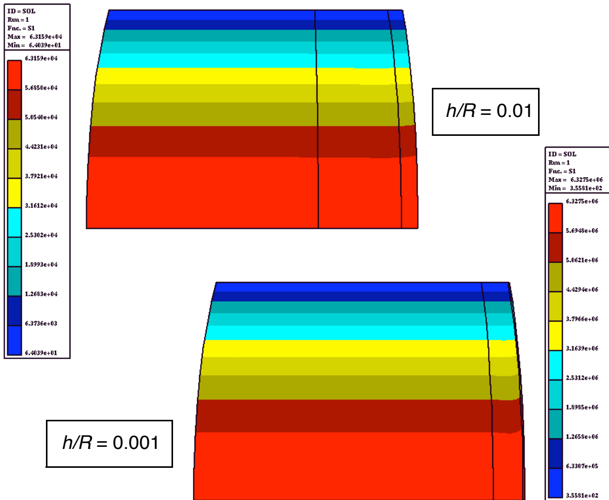
FIGURE 19. Problem 4 - First principal stress distribution at w=h/4 . Shell model 1, Laminated composite case.
