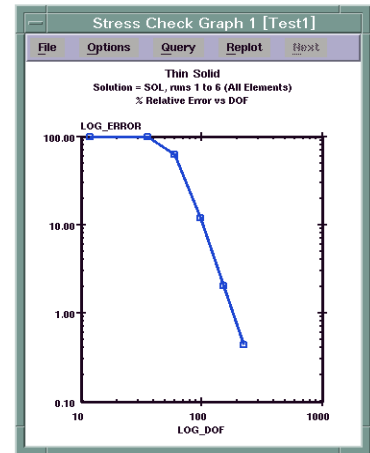
FIGURE 4. Problem 1 - Estimated relative error in energy norm.
