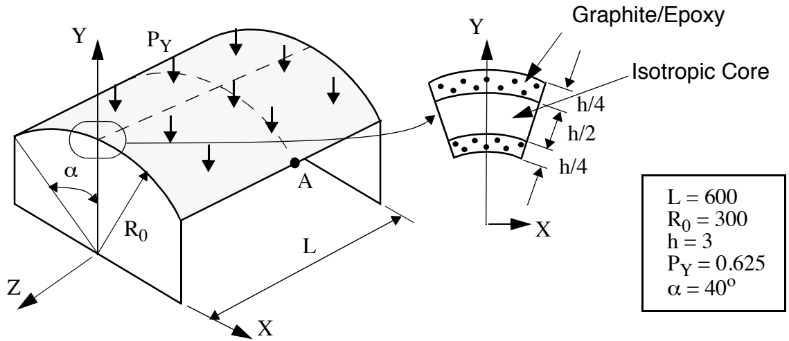
FIGURE 6. Problem 2- Cylindrical roof structure. Notation.
