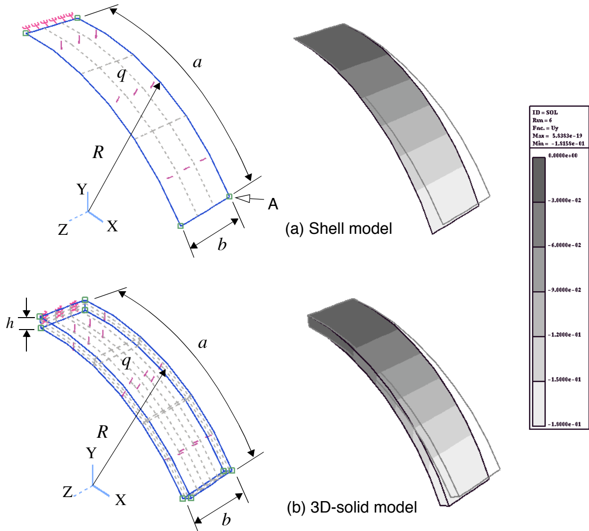
FIGURE 3. Problem 1 - Mesh and contour plot for the shell and 3D-solid models.
