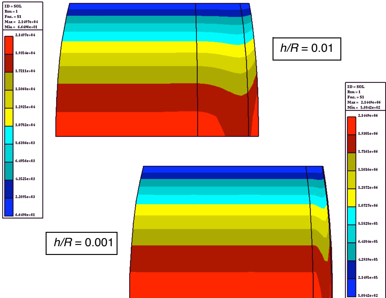
FIGURE 17. Problem 4 - First principal stress distribution at w=h/2 . Shell model 1, isotropic case.
