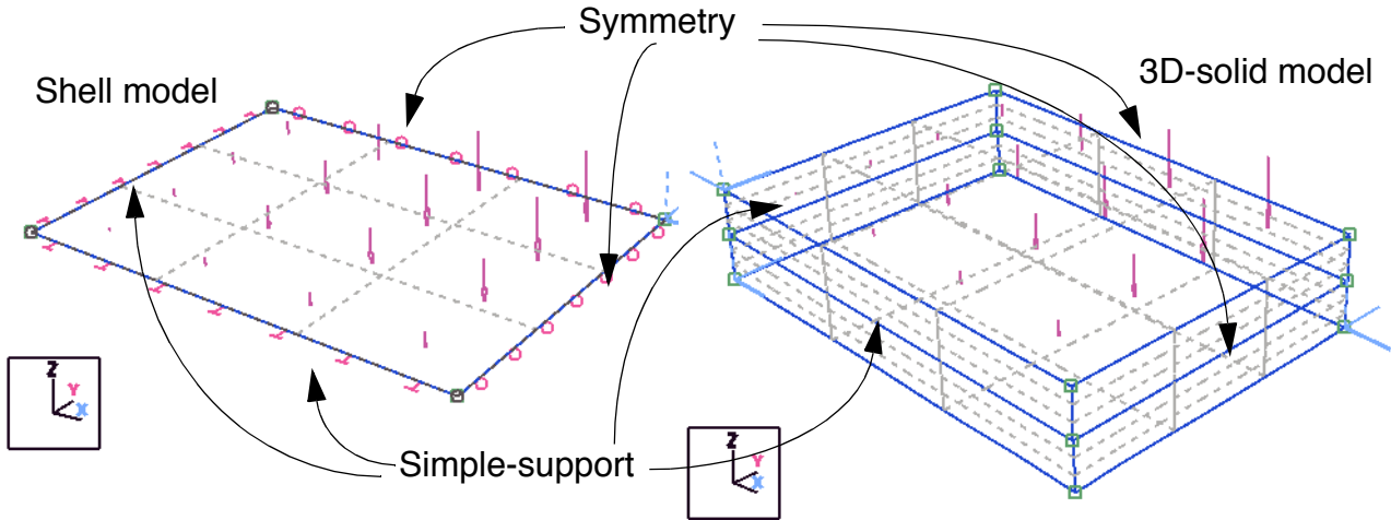
FIGURE 10. Problem 3 - Finite element meshes for the shell and 3D-solid models.
