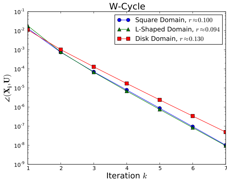
Figure 22: Convergence of the angle between the iterates and the exact eigenvectors using a W-cycle to solve the eigenvalue problem on various domains.
