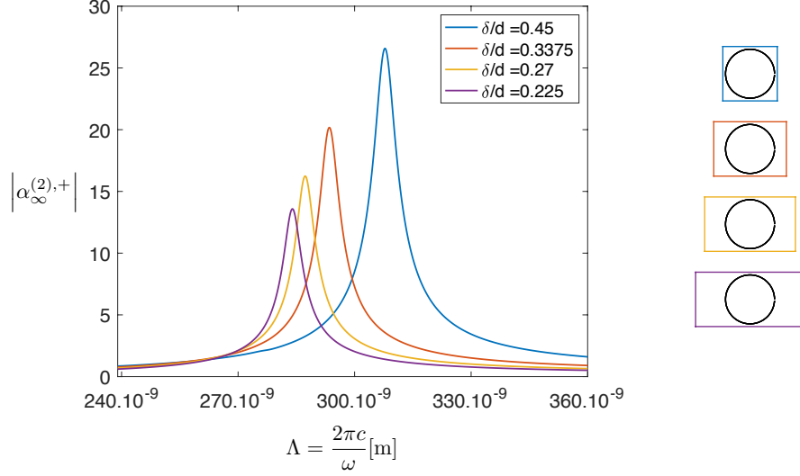
Figure 3 – |\alpha_{\infty}^{(2),+}| as a function of the wavelength for linearly increasing unit cell sizes, from d = 1 (blue contour) to d = 2 (purple contour), with a fixed radius \delta = 0.45 . Water was used for the homogeneous medium ( \varepsilon_m = (1.77)^2 \varepsilon_0 ) and gold for the nanoparticles. For the plasma frequency and damping factor we used T = 10^{-14} \text{s} and \omega_p = 2 \cdot 10^{15} \text{s}^{-1} .
