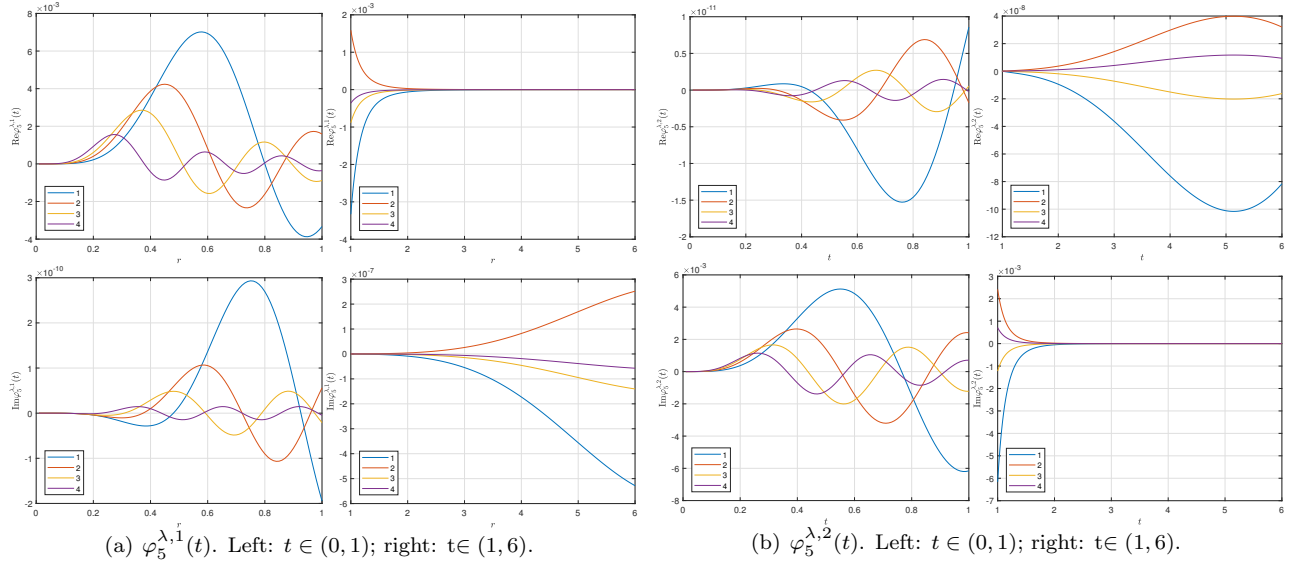
Figure 2: Propagating function \varphi_5^{\lambda,i} for the first four \lambda from \sigma_5^i , i = 1, 2 . First row: real part of \varphi_5^{\lambda,i} ; second row: imaginary part of \varphi_5^{\lambda,i} , for i = 1, 2 .
