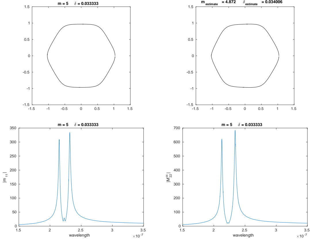
Figure 4.3: From top to bottom and left to right: initial shape, reconstructed shape, |m_{11}| and |M_{22}^{cc}| with respect to the wavelength for m = 5 and \delta = 0.033333 .
