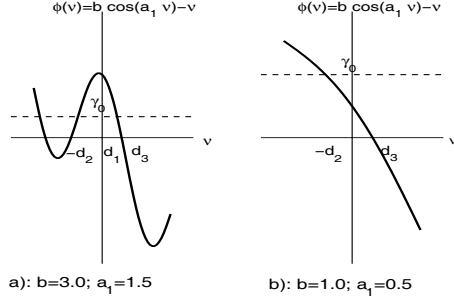
Figure 2: Calculation of the width of the analyticity strip.
