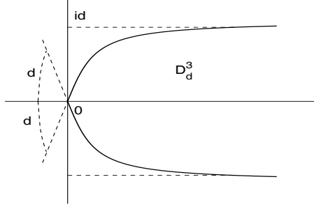
Figure 3: The region \mathcal{D}_d
