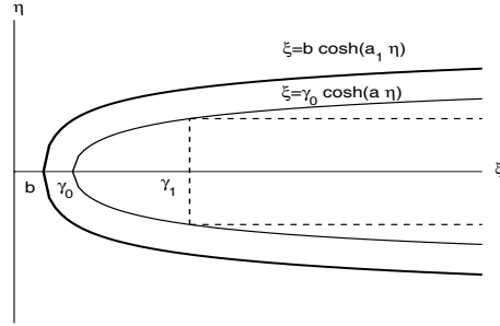
Figure 1: The spectral curve \Gamma_S and the integration curve \Gamma_I .
